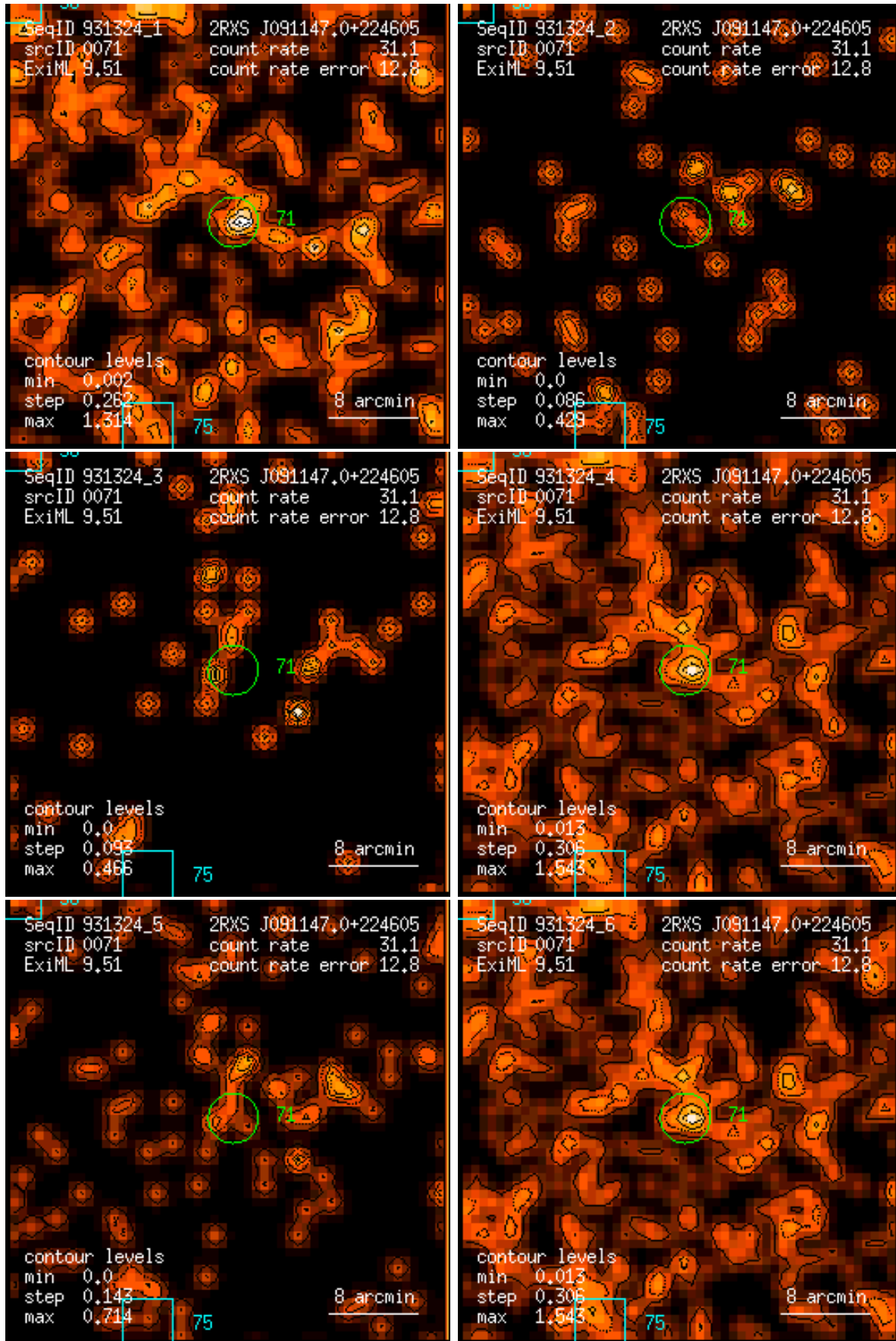
Figure 71: RASS 931324: detection 0071: band rate images, Gaussian filter: (1) PSPC channels 11 – 41, (2) 52 – 90, (3) 91 – 201, (4) 11 – 235, (5) 52 – 201, (6) 11 – 201. Broad band rates in counts/ks. Band rate contour levels in counts/ks/arcmin 2 .
