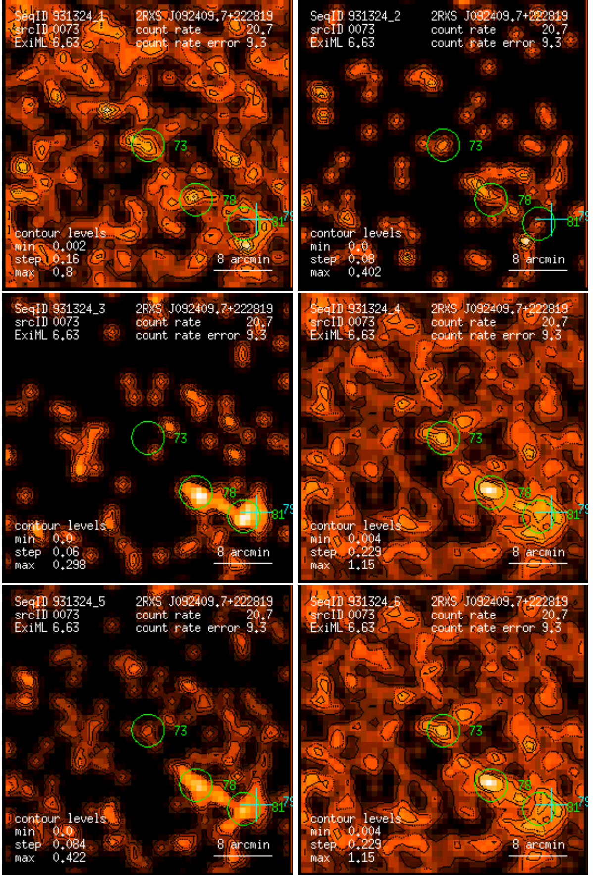
Figure 73: RASS 931324: detection 0073: band rate images, Gaussian filter: (1) PSPC channels 11 – 41, (2) 52 – 90, (3) 91 – 201, (4) 11 – 235, (5) 52 – 201, (6) 11 – 201. Broad band rates in counts/ks. Band rate contour levels in counts/ks/arcmin 2 .
