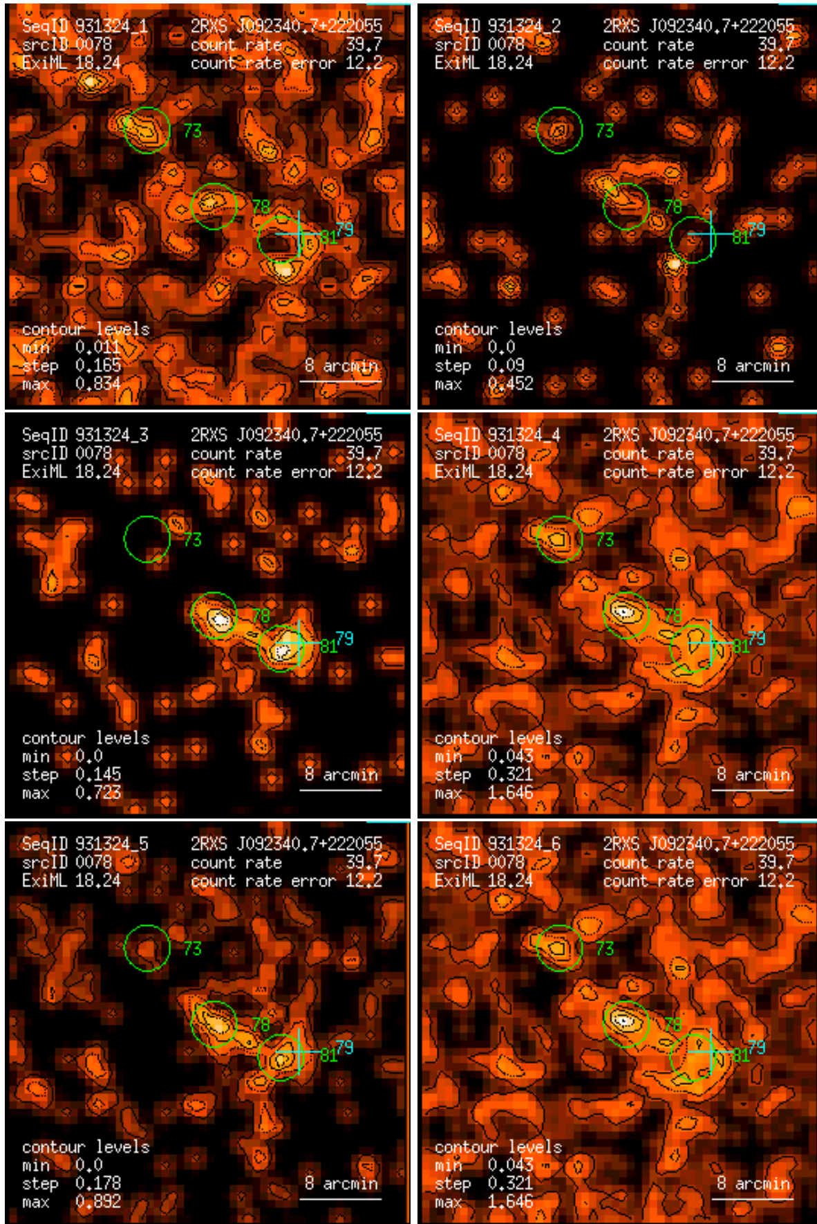
Figure 78: RASS 931324: detection 0078: band rate images, Gaussian filter: (1) PSPC channels 11 – 41, (2) 52 – 90, (3) 91 – 201, (4) 11 – 235, (5) 52 – 201, (6) 11 – 201. Broad band rates in counts/ks. Band rate contour levels in counts/ks/arcmin 2 .
