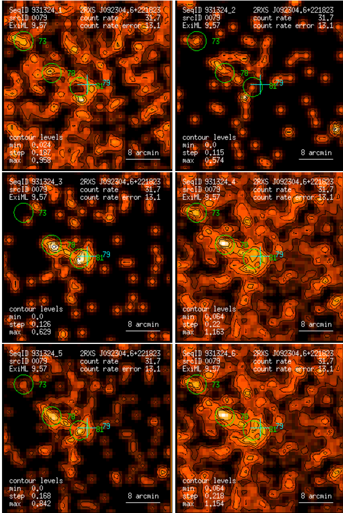
Figure 79: RASS 931324: detection 0079: band rate images, Gaussian filter: (1) PSPC channels 11 – 41, (2) 52 – 90, (3) 91 – 201, (4) 11 – 235, (5) 52 – 201, (6) 11 – 201. Broad band rates in counts/ks. Band rate contour levels in counts/ks/arcmin 2 .
