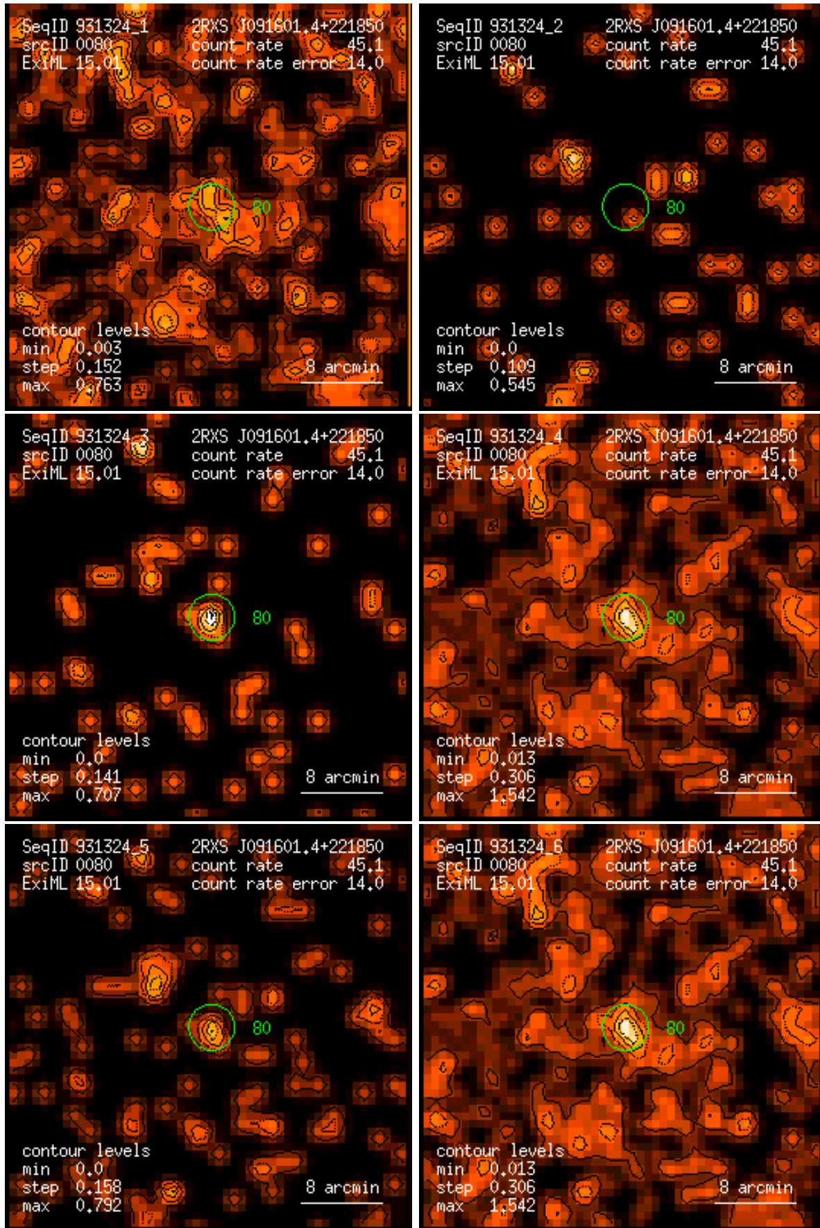
Figure 80: RASS 931324: detection 0080: band rate images, Gaussian filter: (1) PSPC channels 11 – 41, (2) 52 – 90, (3) 91 – 201, (4) 11 – 235, (5) 52 – 201, (6) 11 – 201. Broad band rates in counts/ks. Band rate contour levels in counts/ks/arcmin 2 .
