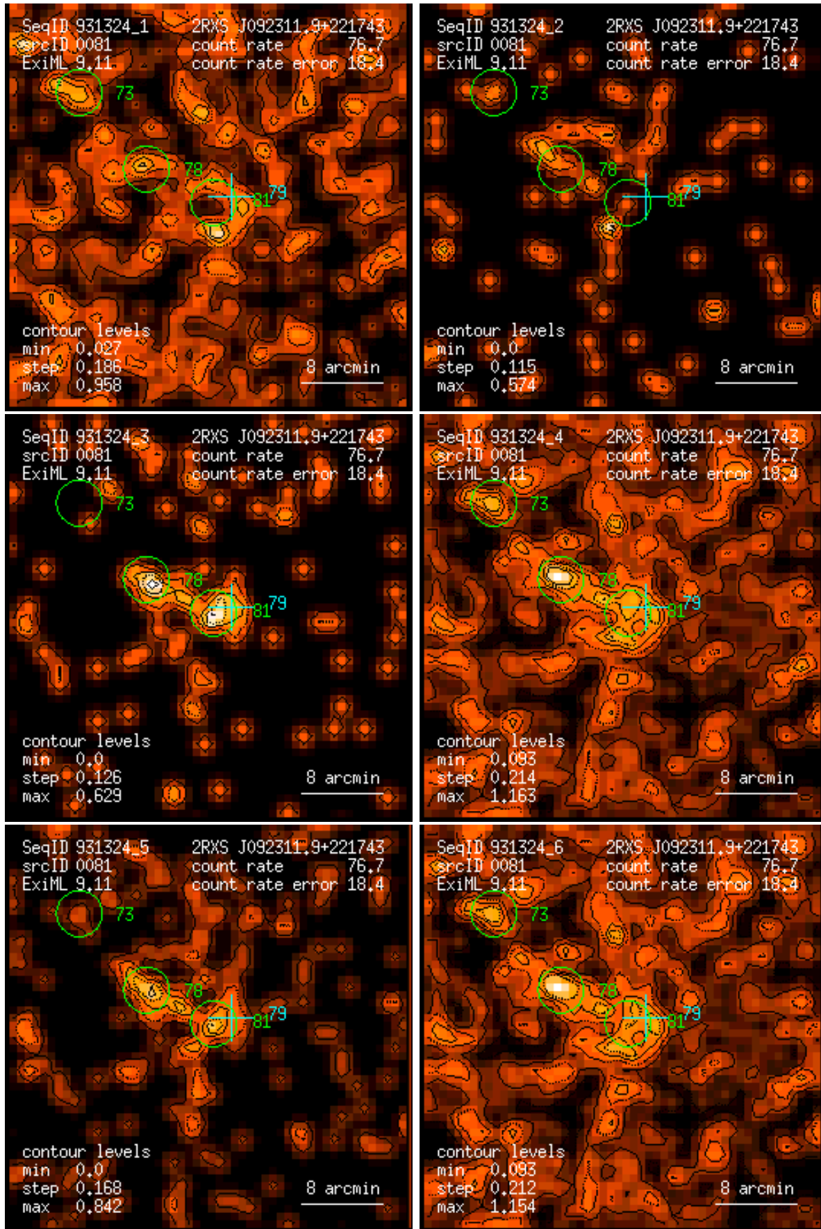
Figure 81: RASS 931324: detection 0081: band rate images, Gaussian filter: (1) PSPC channels 11 – 41, (2) 52 – 90, (3) 91 – 201, (4) 11 – 235, (5) 52 – 201, (6) 11 – 201. Broad band rates in counts/ks. Band rate contour levels in counts/ks/arcmin 2 .
