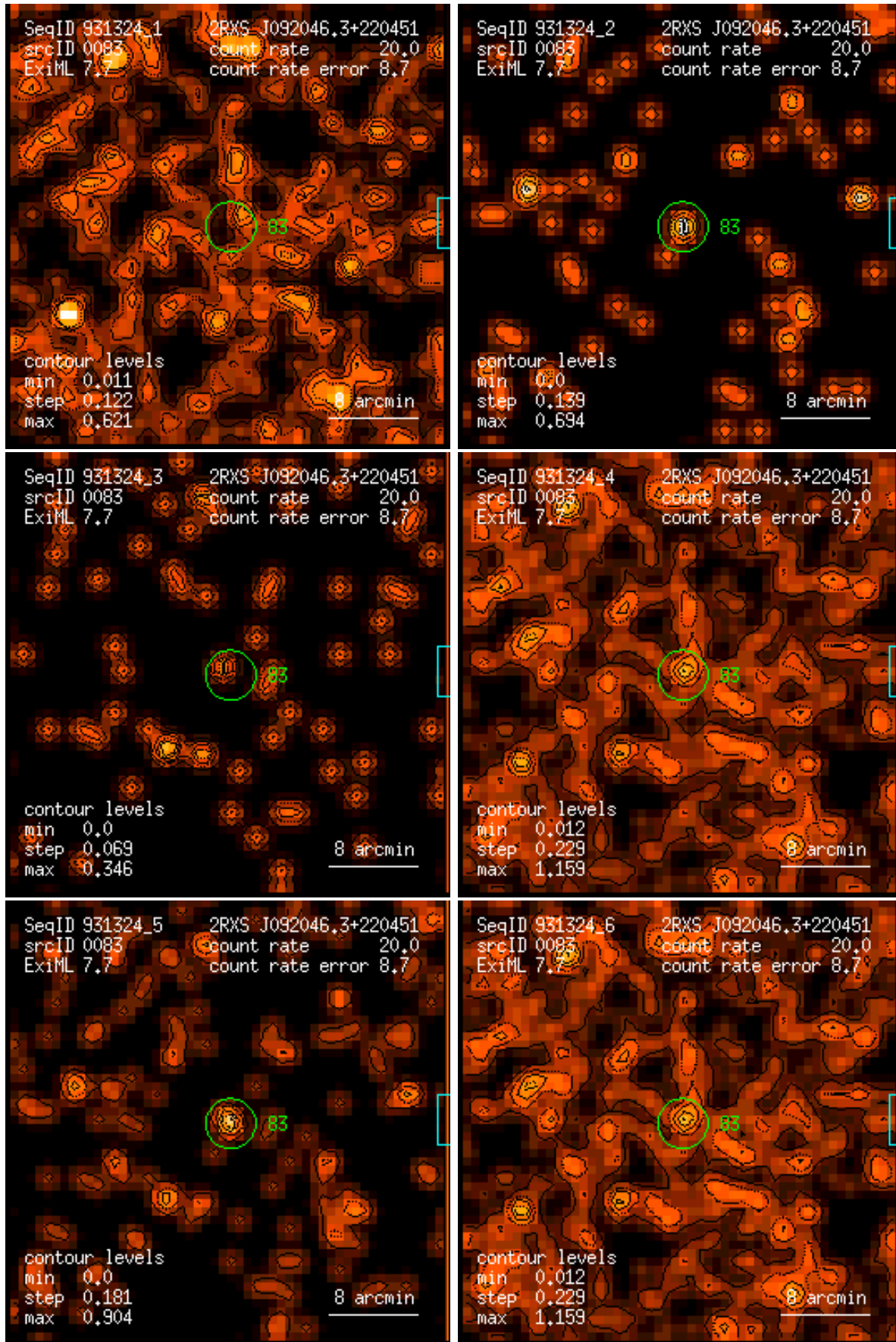
Figure 83: RASS 931324: detection 0083: band rate images, Gaussian filter: (1) PSPC channels 11 – 41, (2) 52 – 90, (3) 91 – 201, (4) 11 – 235, (5) 52 – 201, (6) 11 – 201. Broad band rates in counts/ks. Band rate contour levels in counts/ks/arcmin 2 .
