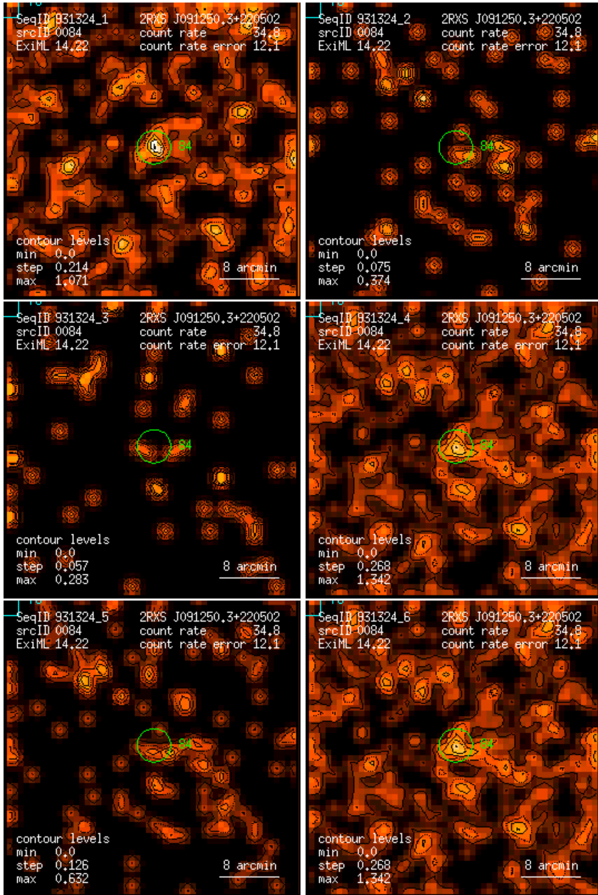
Figure 84: RASS 931324: detection 0084: band rate images, Gaussian filter: (1) PSPC channels 11 – 41, (2) 52 – 90, (3) 91 – 201, (4) 11 – 235, (5) 52 – 201, (6) 11 – 201. Broad band rates in counts/ks. Band rate contour levels in counts/ks/arcmin 2 .
