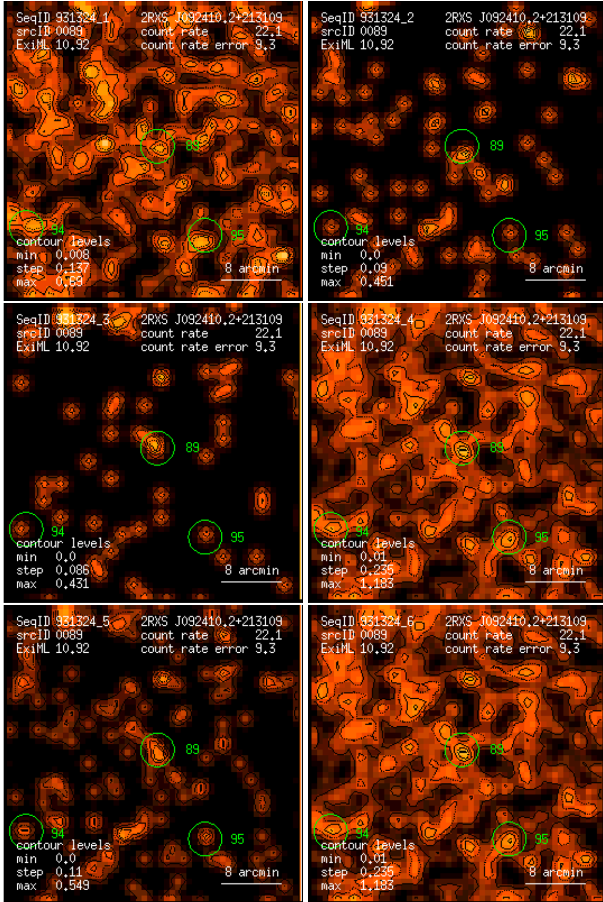
Figure 89: RASS 931324: detection 0089: band rate images, Gaussian filter: (1) PSPC channels 11 – 41, (2) 52 – 90, (3) 91 – 201, (4) 11 – 235, (5) 52 – 201, (6) 11 – 201. Broad band rates in counts/ks. Band rate contour levels in counts/ks/arcmin 2 .
