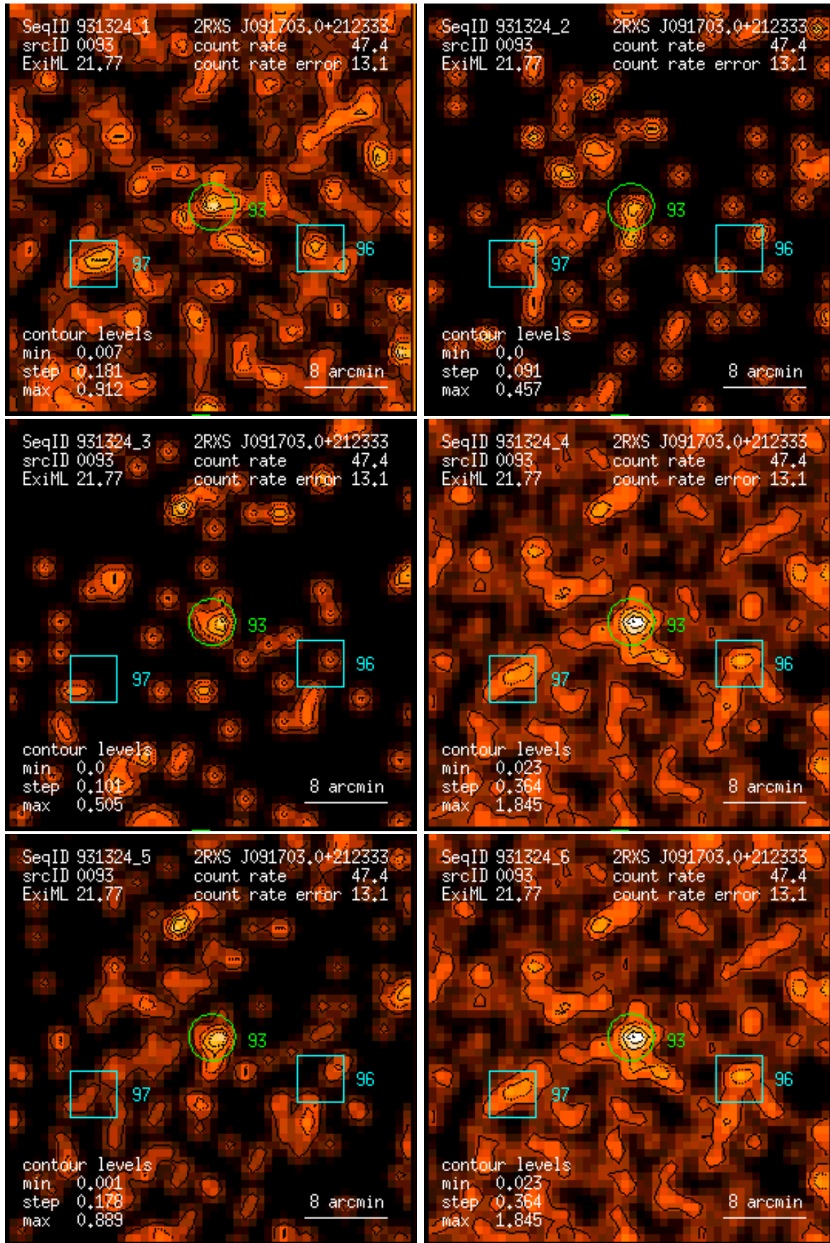
Figure 93: RASS 931324: detection 0093: band rate images, Gaussian filter: (1) PSPC channels 11 – 41, (2) 52 – 90, (3) 91 – 201, (4) 11 – 235, (5) 52 – 201, (6) 11 – 201. Broad band rates in counts/ks. Band rate contour levels in counts/ks/arcmin 2 .
