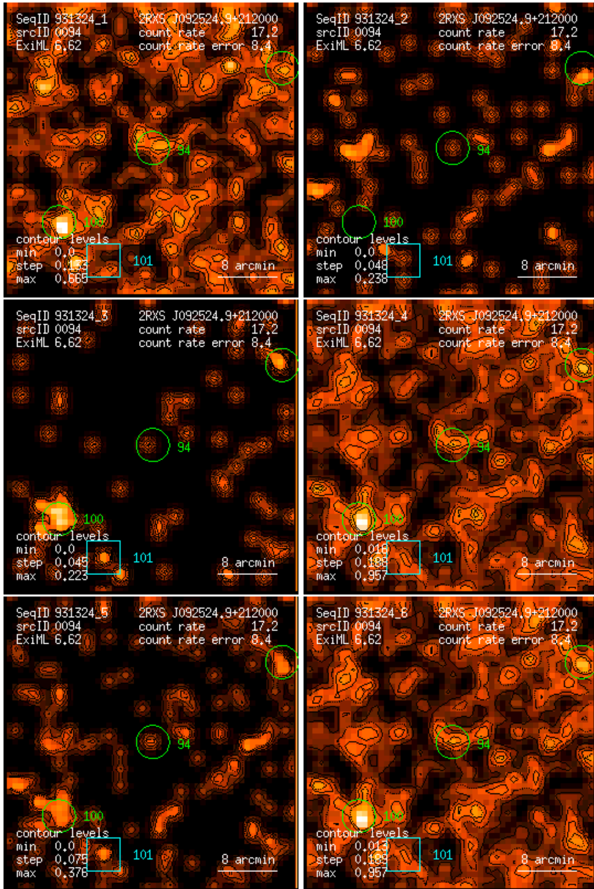
Figure 94: RASS 931324: detection 0094: band rate images, Gaussian filter: (1) PSPC channels 11 – 41, (2) 52 – 90, (3) 91 – 201, (4) 11 – 235, (5) 52 – 201, (6) 11 – 201. Broad band rates in counts/ks. Band rate contour levels in counts/ks/arcmin 2 .
