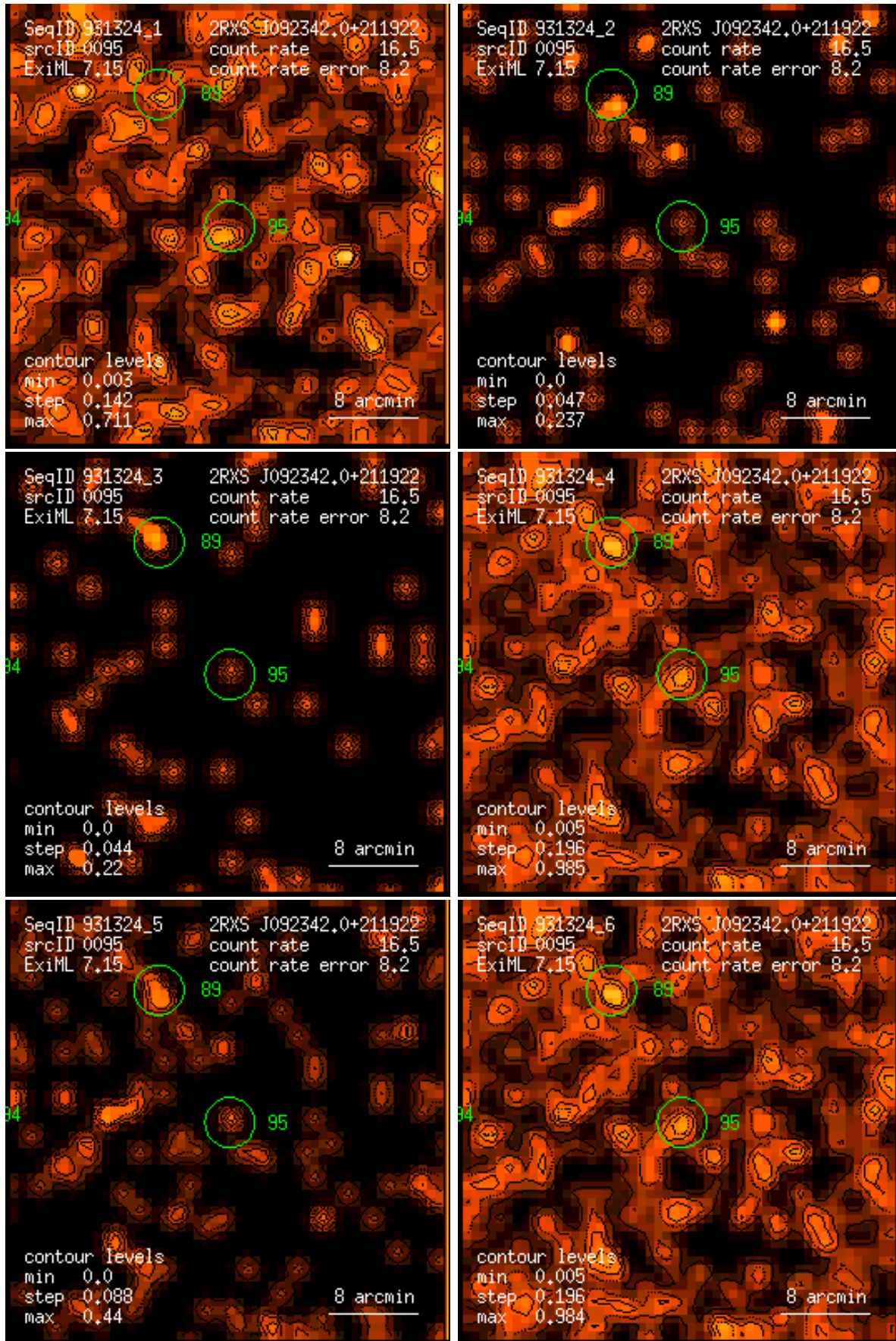
Figure 95: RASS 931324: detection 0095: band rate images, Gaussian filter: (1) PSPC channels 11 – 41, (2) 52 – 90, (3) 91 – 201, (4) 11 – 235, (5) 52 – 201, (6) 11 – 201. Broad band rates in counts/ks. Band rate contour levels in counts/ks/arcmin 2 .
