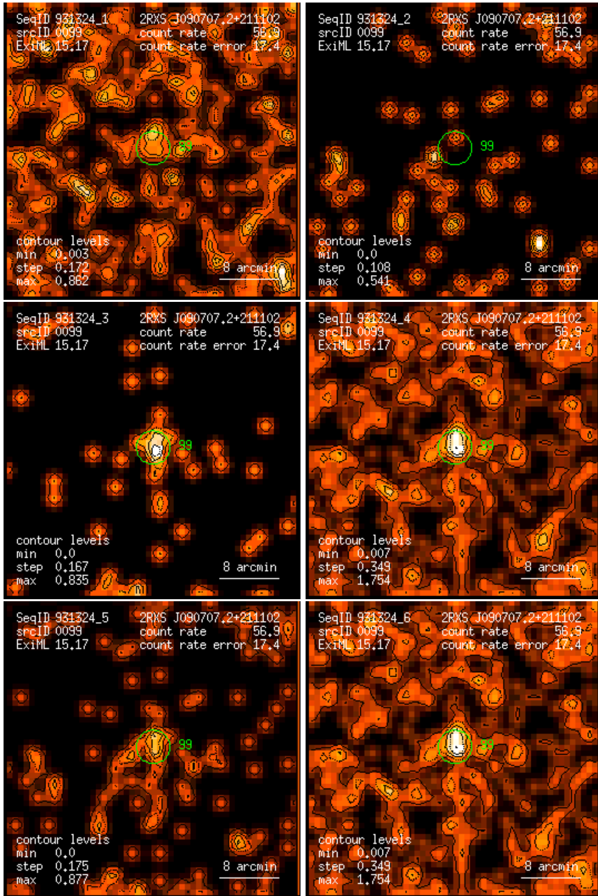
Figure 99: RASS 931324: detection 0099: band rate images, Gaussian filter: (1) PSPC channels 11 – 41, (2) 52 – 90, (3) 91 – 201, (4) 11 – 235, (5) 52 – 201, (6) 11 – 201. Broad band rates in counts/ks. Band rate contour levels in counts/ks/arcmin 2 .
