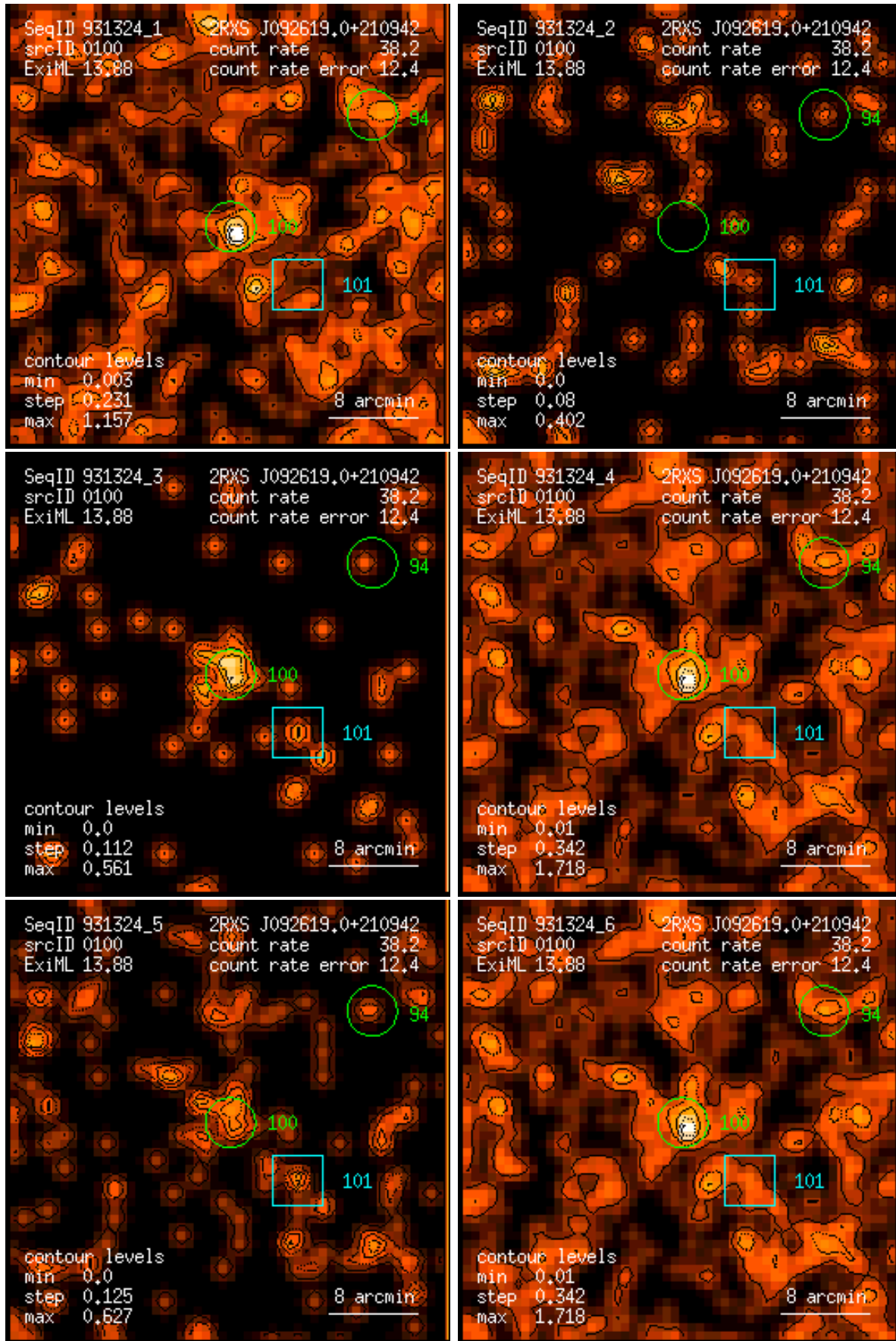
Figure 100: RASS 931324: detection 0100: band rate images, Gaussian filter: (1) PSPC channels 11 – 41, (2) 52 – 90, (3) 91 – 201, (4) 11 – 235, (5) 52 – 201, (6) 11 – 201. Broad band rates in counts/ks. Band rate contour levels in counts/ks/arcmin 2 .
