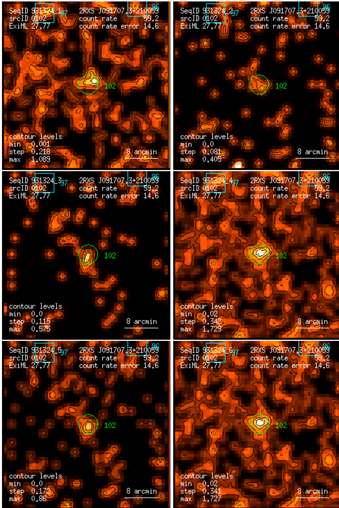
Figure 102: RASS 931324: detection 0102: band rate images, Gaussian filter: (1) PSPC channels 11 – 41, (2) 52 – 90, (3) 91 – 201, (4) 11 – 235, (5) 52 – 201, (6) 11 – 201. Broad band rates in counts/ks. Band rate contour levels in counts/ks/arcmin 2 .
