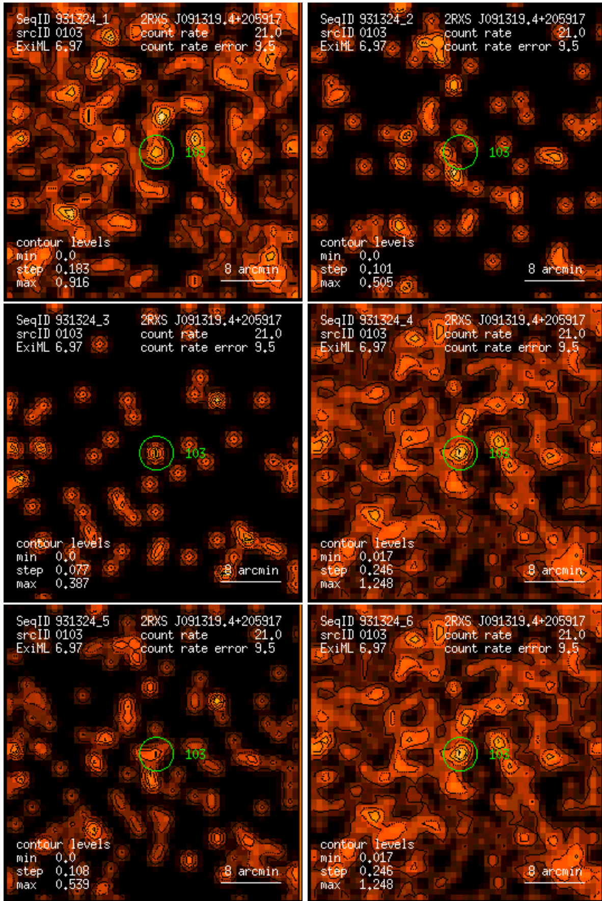
Figure 103: RASS 931324: detection 0103: band rate images, Gaussian filter: (1) PSPC channels 11 – 41, (2) 52 – 90, (3) 91 – 201, (4) 11 – 235, (5) 52 – 201, (6) 11 – 201. Broad band rates in counts/ks. Band rate contour levels in counts/ks/arcmin 2 .
