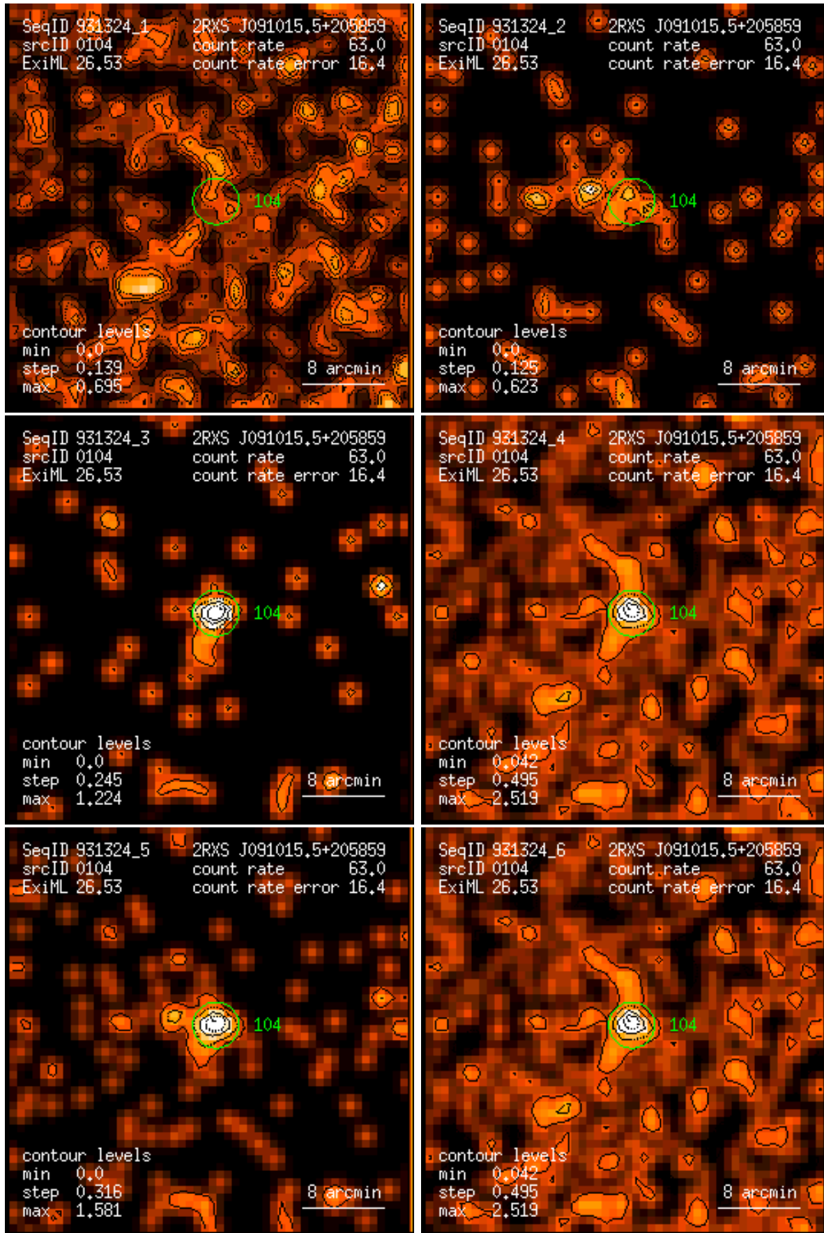
Figure 104: RASS 931324: detection 0104: band rate images, Gaussian filter: (1) PSPC channels 11 – 41, (2) 52 – 90, (3) 91 – 201, (4) 11 – 235, (5) 52 – 201, (6) 11 – 201. Broad band rates in counts/ks. Band rate contour levels in counts/ks/arcmin 2 .
