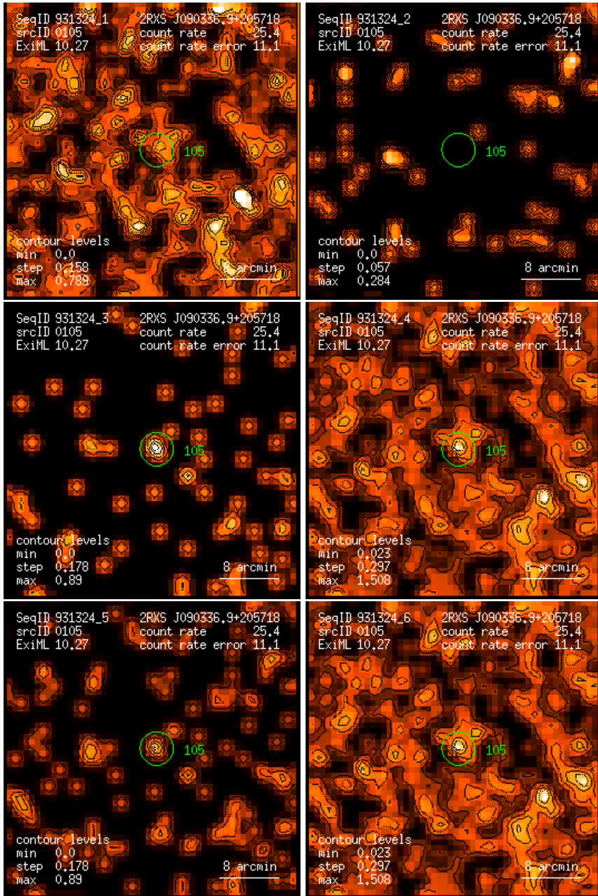
Figure 105: RASS 931324: detection 0105: band rate images, Gaussian filter: (1) PSPC channels 11 – 41, (2) 52 – 90, (3) 91 – 201, (4) 11 – 235, (5) 52 – 201, (6) 11 – 201. Broad band rates in counts/ks. Band rate contour levels in counts/ks/arcmin 2 .
