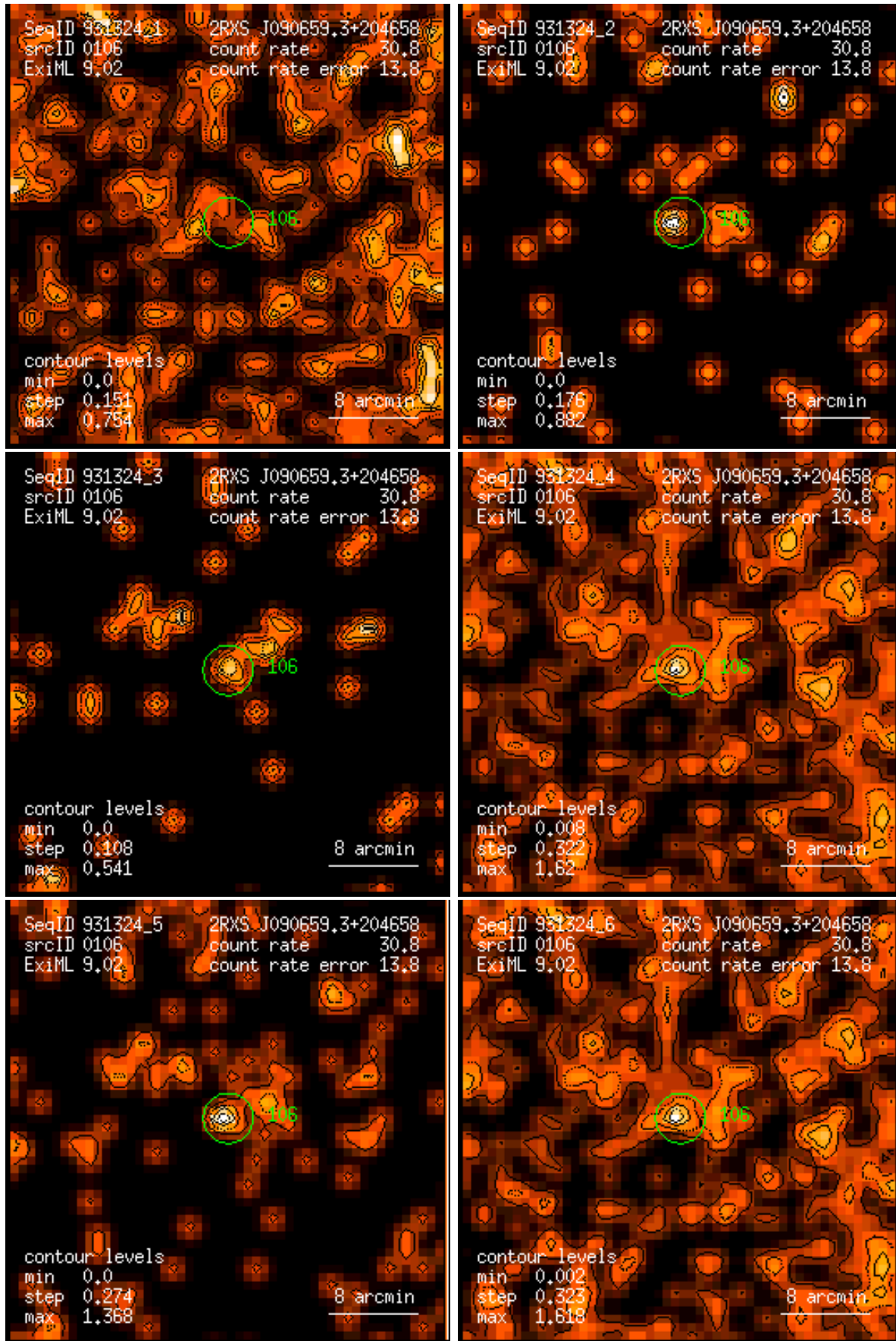
Figure 106: RASS 931324: detection 0106: band rate images, Gaussian filter: (1) PSPC channels 11 – 41, (2) 52 – 90, (3) 91 – 201, (4) 11 – 235, (5) 52 – 201, (6) 11 – 201. Broad band rates in counts/ks. Band rate contour levels in counts/ks/arcmin 2 .
