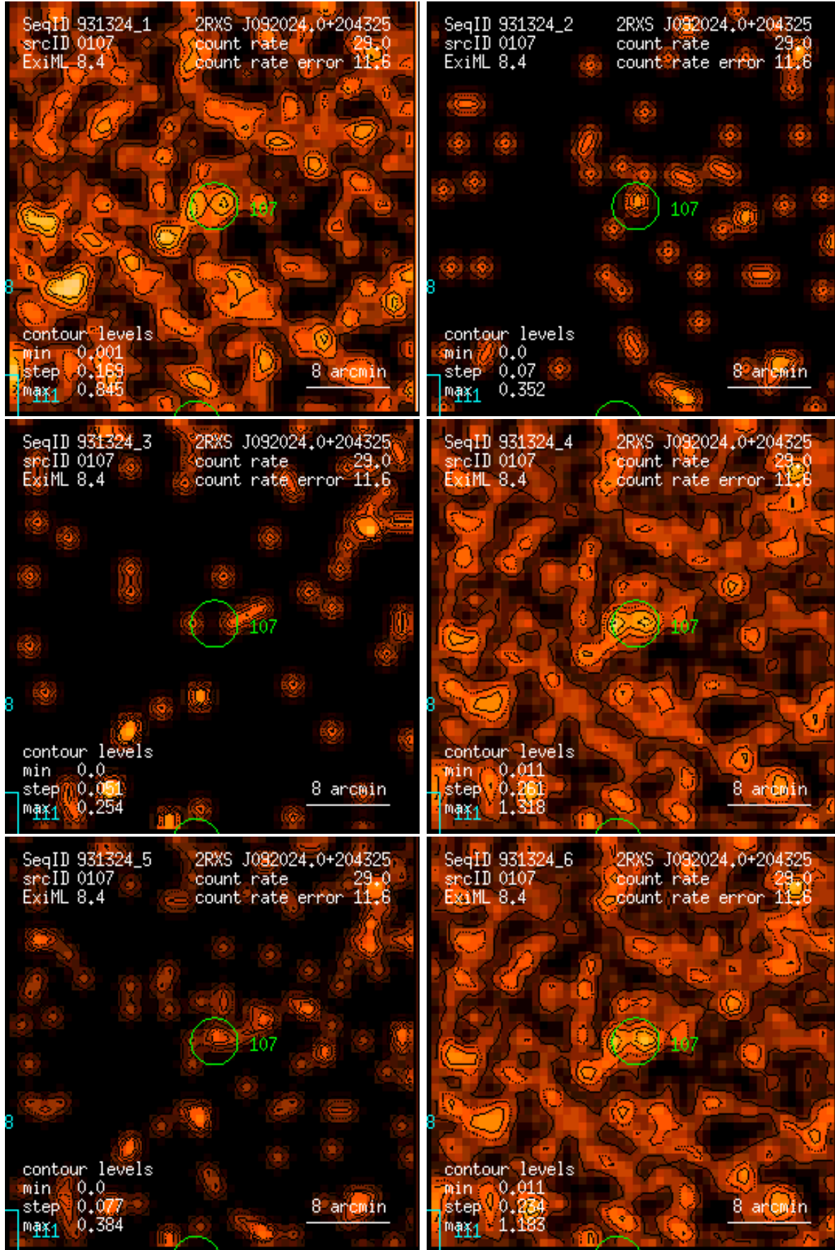
Figure 107: RASS 931324: detection 0107: band rate images, Gaussian filter: (1) PSPC channels 11 – 41, (2) 52 – 90, (3) 91 – 201, (4) 11 – 235, (5) 52 – 201, (6) 11 – 201. Broad band rates in counts/ks. Band rate contour levels in counts/ks/arcmin 2 .
