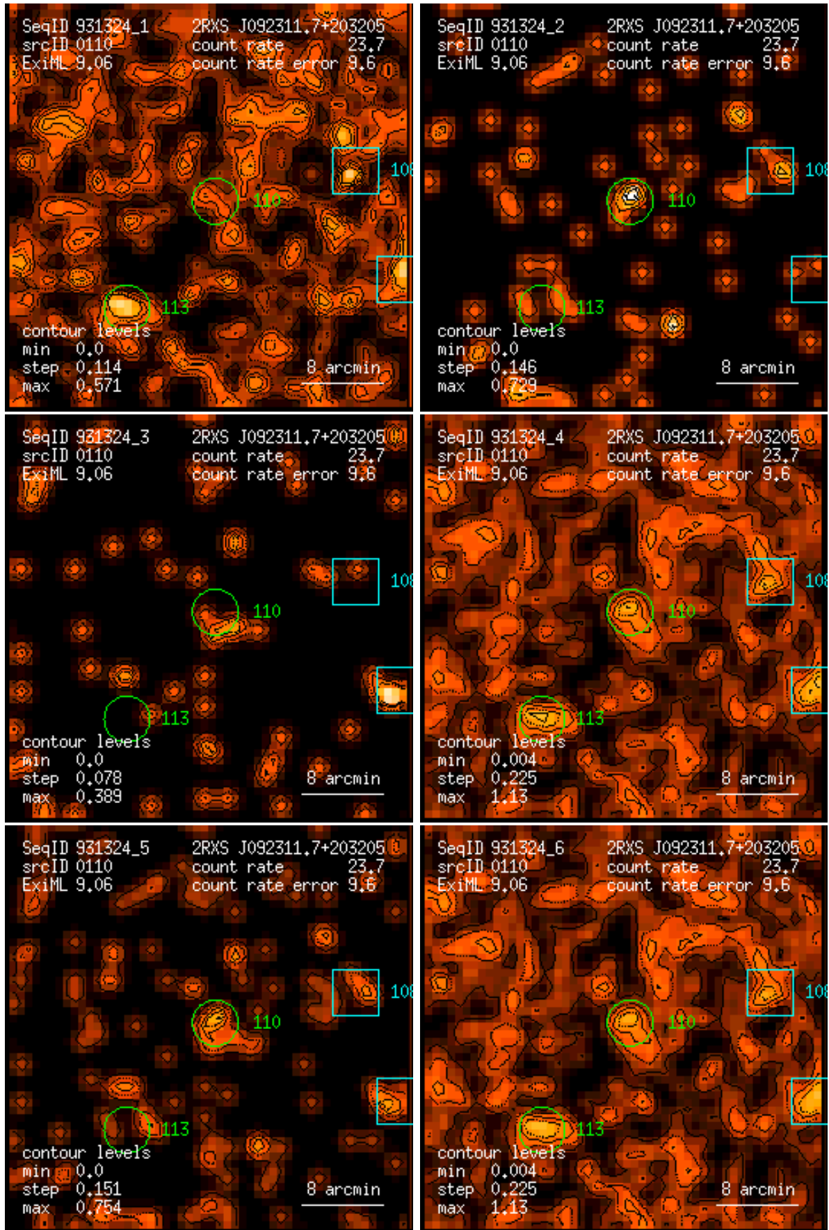
Figure 110: RASS 931324: detection 0110: band rate images, Gaussian filter: (1) PSPC channels 11 – 41, (2) 52 – 90, (3) 91 – 201, (4) 11 – 235, (5) 52 – 201, (6) 11 – 201. Broad band rates in counts/ks. Band rate contour levels in counts/ks/arcmin 2 .
