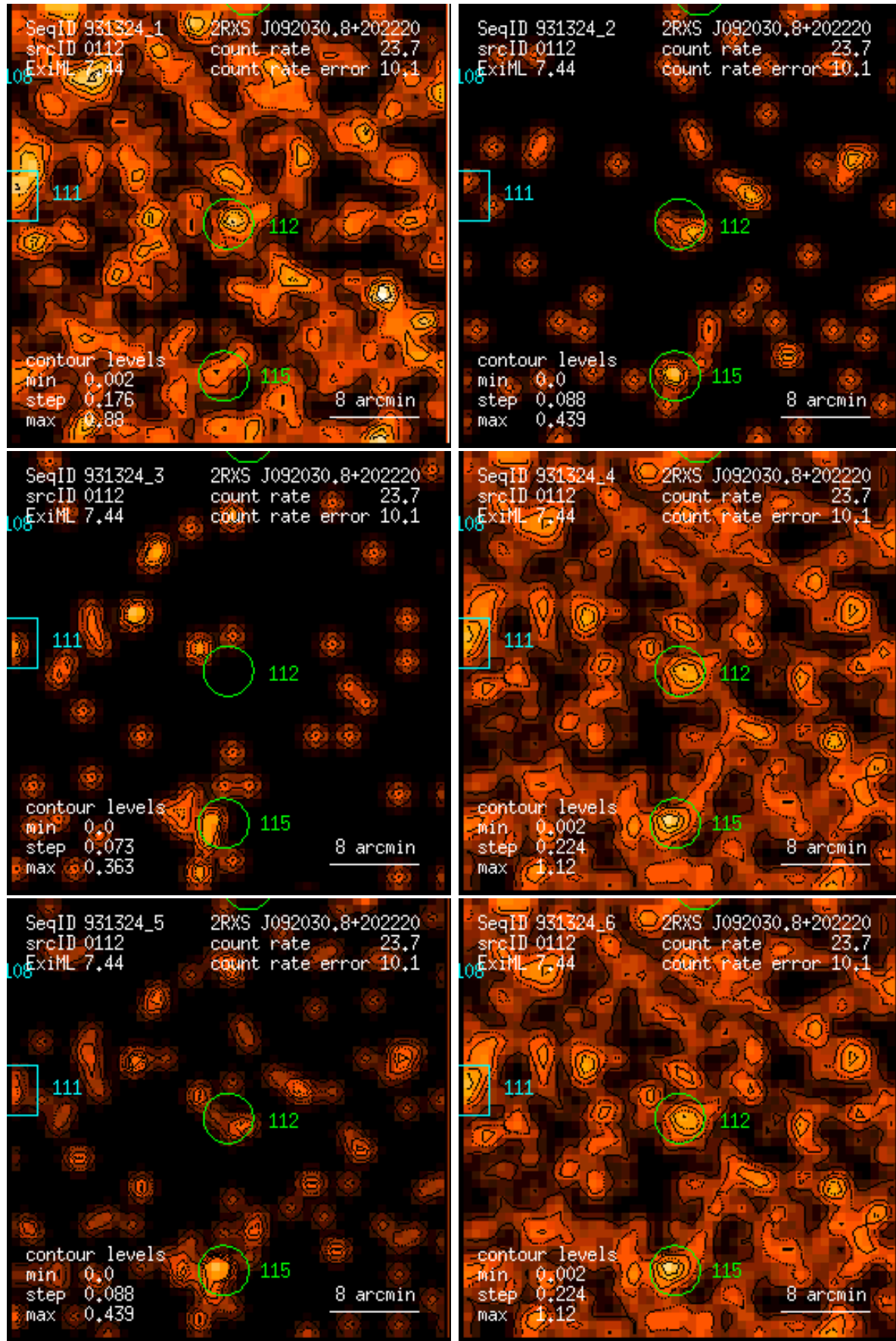
Figure 112: RASS 931324: detection 0112: band rate images, Gaussian filter: (1) PSPC channels 11 – 41, (2) 52 – 90, (3) 91 – 201, (4) 11 – 235, (5) 52 – 201, (6) 11 – 201. Broad band rates in counts/ks. Band rate contour levels in counts/ks/arcmin 2 .
