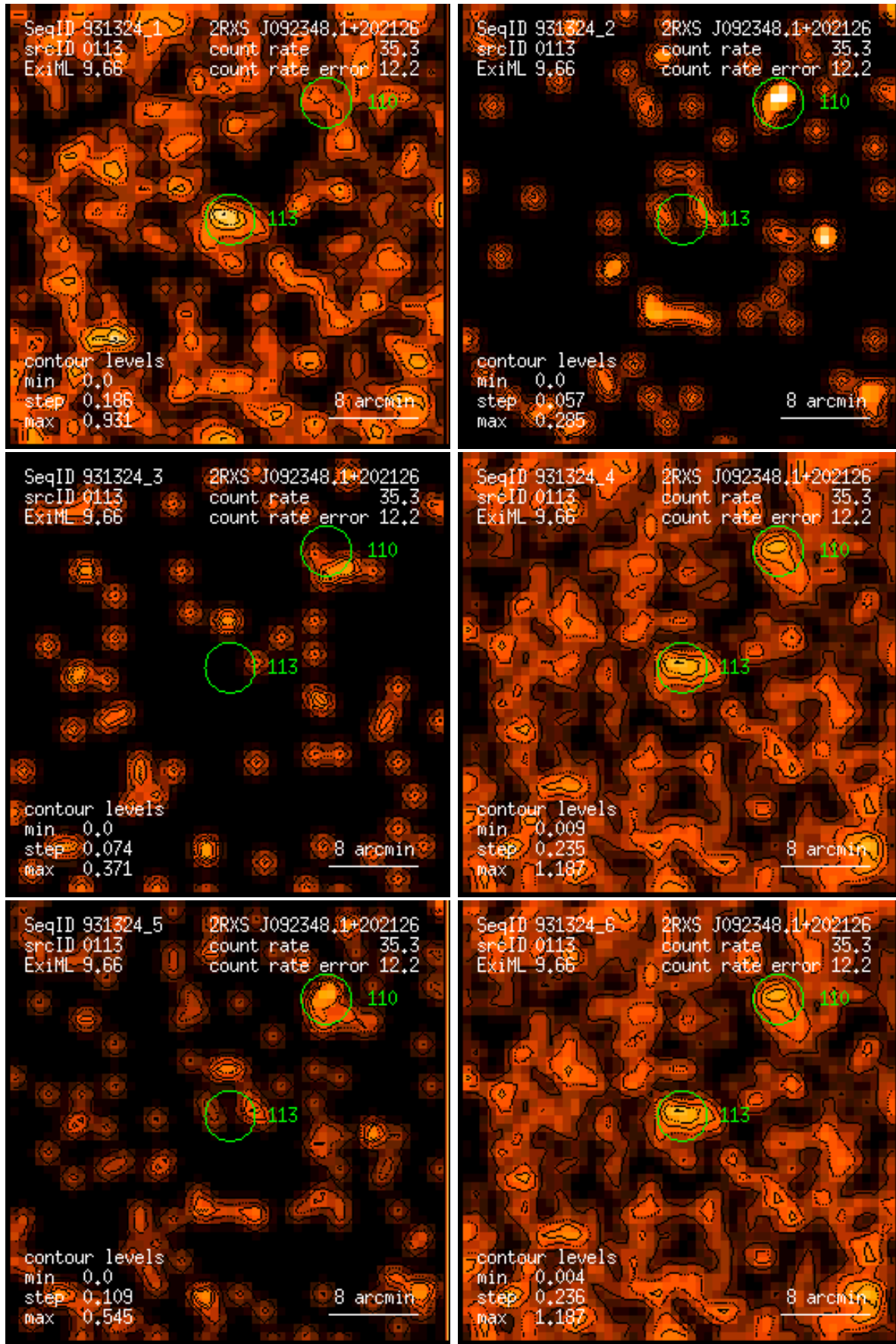
Figure 113: RASS 931324: detection 0113: band rate images, Gaussian filter: (1) PSPC channels 11 – 41, (2) 52 – 90, (3) 91 – 201, (4) 11 – 235, (5) 52 – 201, (6) 11 – 201. Broad band rates in counts/ks. Band rate contour levels in counts/ks/arcmin 2 .
