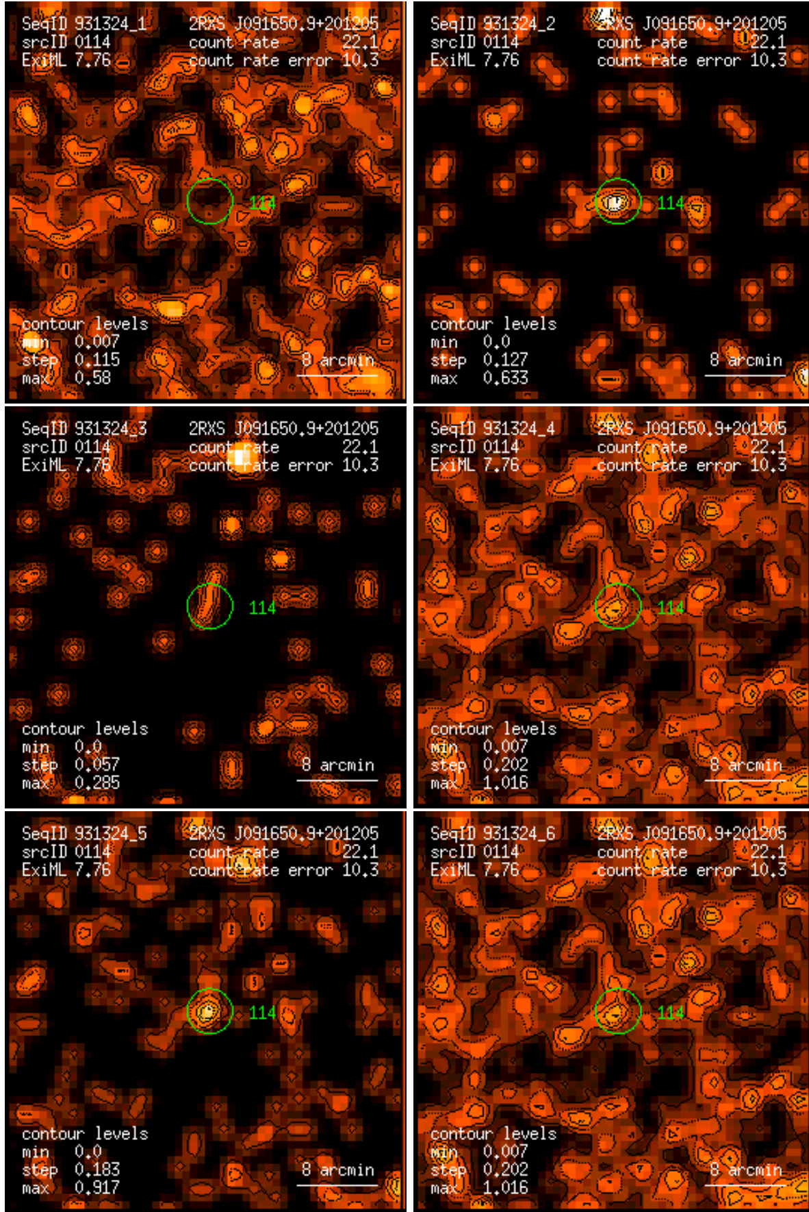
Figure 114: RASS 931324: detection 0114: band rate images, Gaussian filter: (1) PSPC channels 11 – 41, (2) 52 – 90, (3) 91 – 201, (4) 11 – 235, (5) 52 – 201, (6) 11 – 201. Broad band rates in counts/ks. Band rate contour levels in counts/ks/arcmin 2 .
