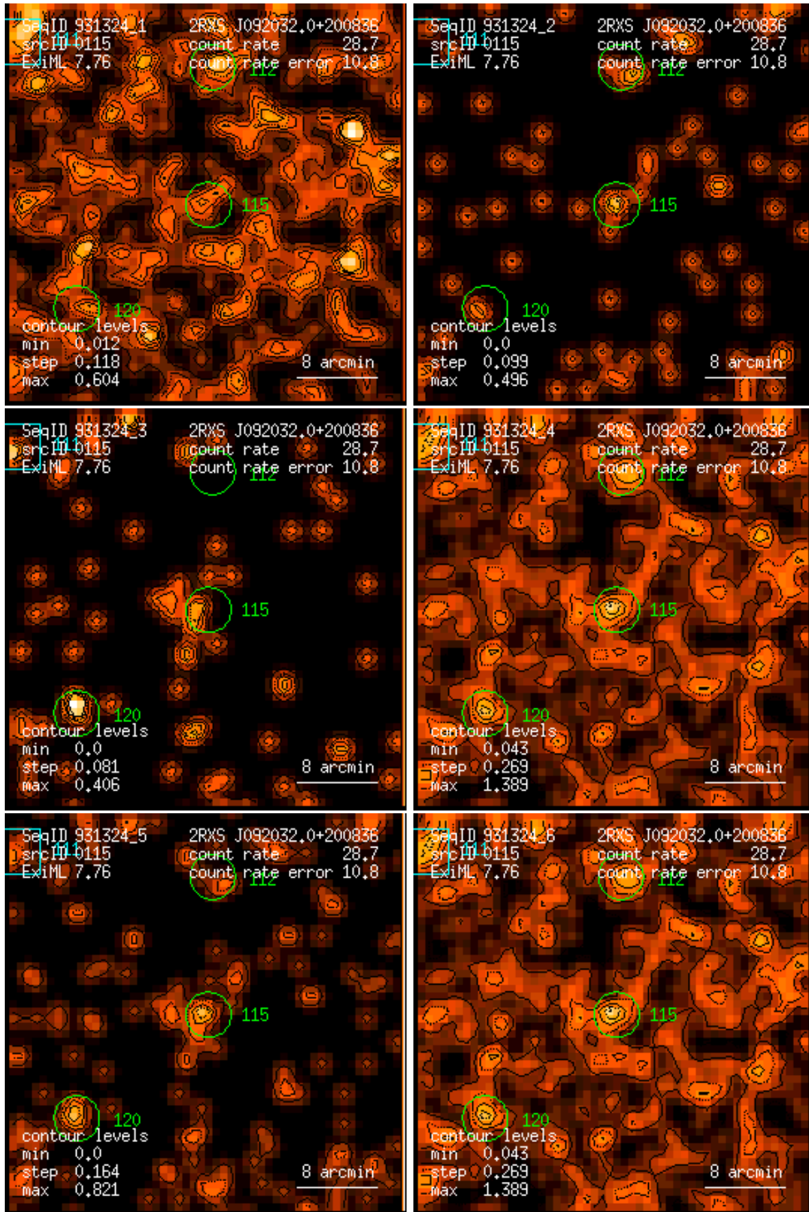
Figure 115: RASS 931324: detection 0115: band rate images, Gaussian filter: (1) PSPC channels 11 – 41, (2) 52 – 90, (3) 91 – 201, (4) 11 – 235, (5) 52 – 201, (6) 11 – 201. Broad band rates in counts/ks. Band rate contour levels in counts/ks/arcmin 2 .
