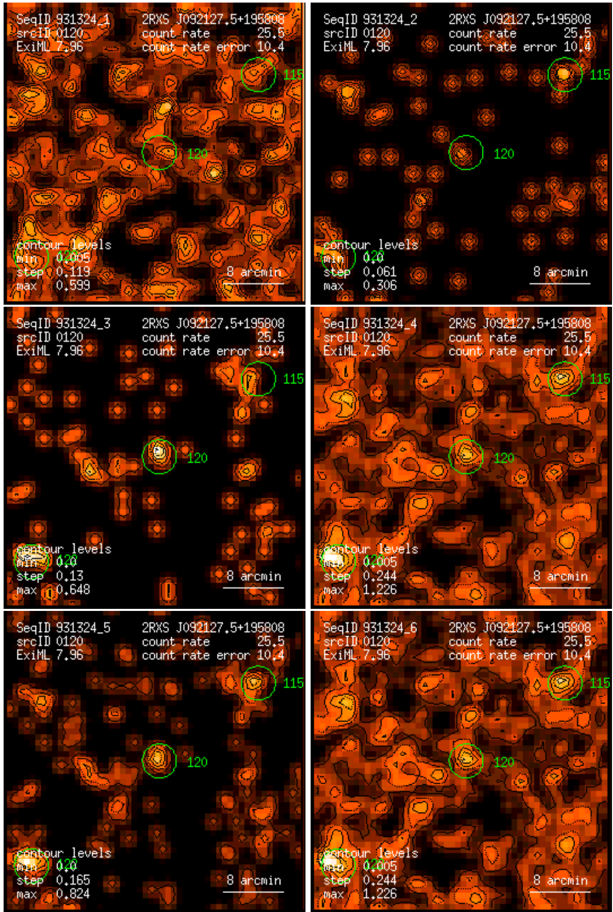
Figure 120: RASS 931324: detection 0120: band rate images, Gaussian filter: (1) PSPC channels 11 – 41, (2) 52 – 90, (3) 91 – 201, (4) 11 – 235, (5) 52 – 201, (6) 11 – 201. Broad band rates in counts/ks. Band rate contour levels in counts/ks/arcmin 2 .
