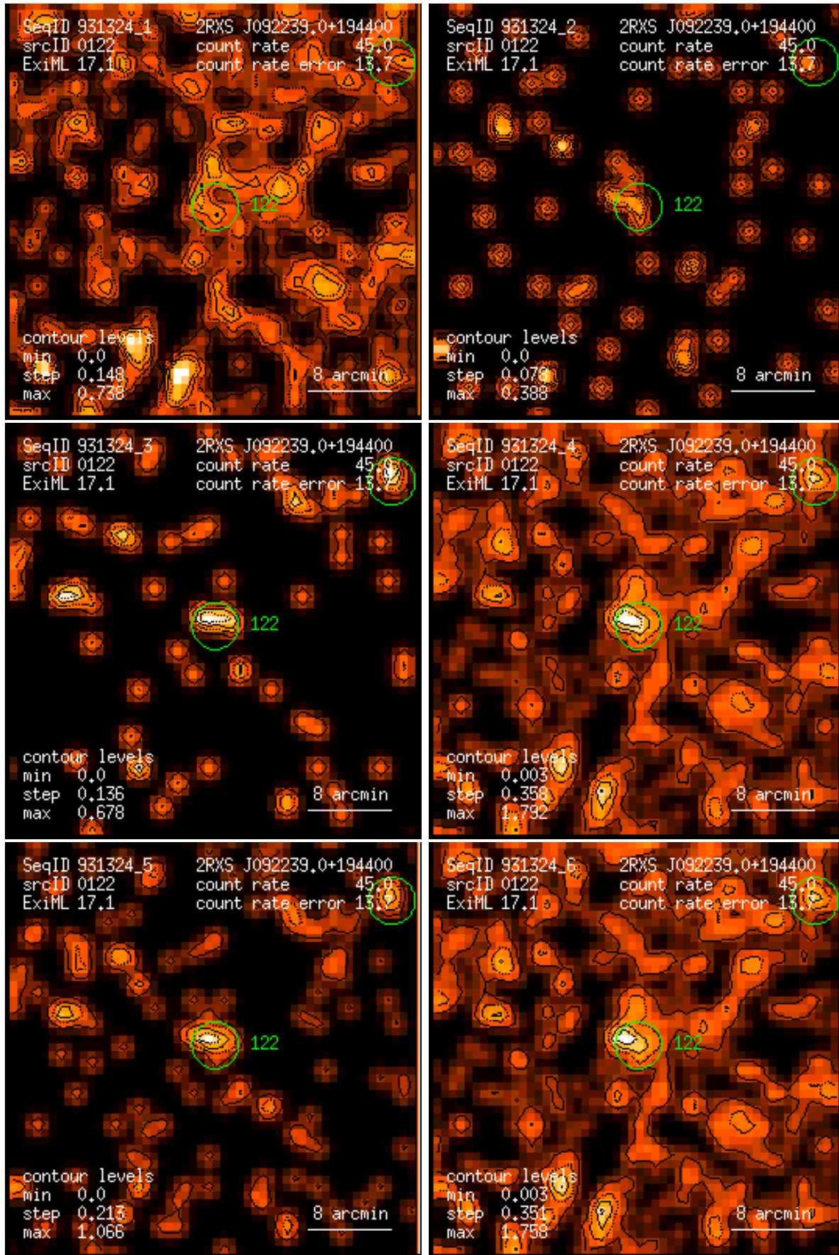
Figure 122: RASS 931324: detection 0122: band rate images, Gaussian filter: (1) PSPC channels 11 – 41, (2) 52 – 90, (3) 91 – 201, (4) 11 – 235, (5) 52 – 201, (6) 11 – 201. Broad band rates in counts/ks. Band rate contour levels in counts/ks/arcmin 2 .
