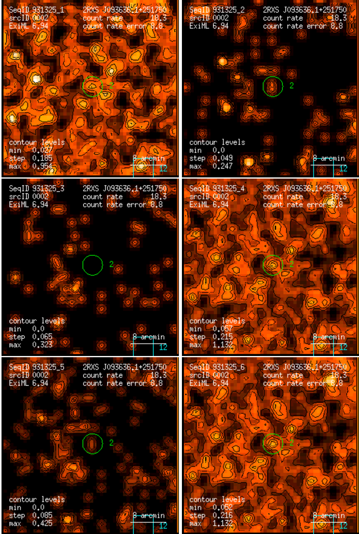
Figure 2: RASS 931325: detection 0002: band rate images, Gaussian filter: (1) PSPC channels 11 – 41, (2) 52 – 90, (3) 91 – 201, (4) 11 – 235, (5) 52 – 201, (6) 11 – 201. Broad band rates in counts/ks. Band rate contour levels in counts/ks/arcmin 2 .
