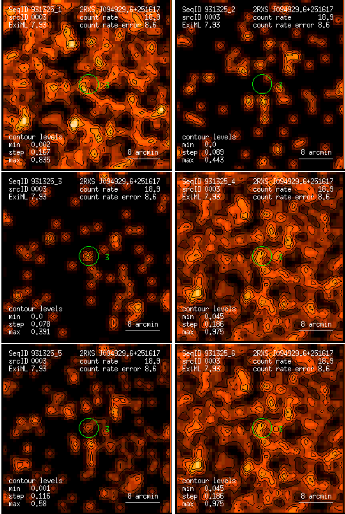
Figure 3: RASS 931325: detection 0003: band rate images, Gaussian filter: (1) PSPC channels 11 – 41, (2) 52 – 90, (3) 91 – 201, (4) 11 – 235, (5) 52 – 201, (6) 11 – 201. Broad band rates in counts/ks. Band rate contour levels in counts/ks/arcmin 2 .
