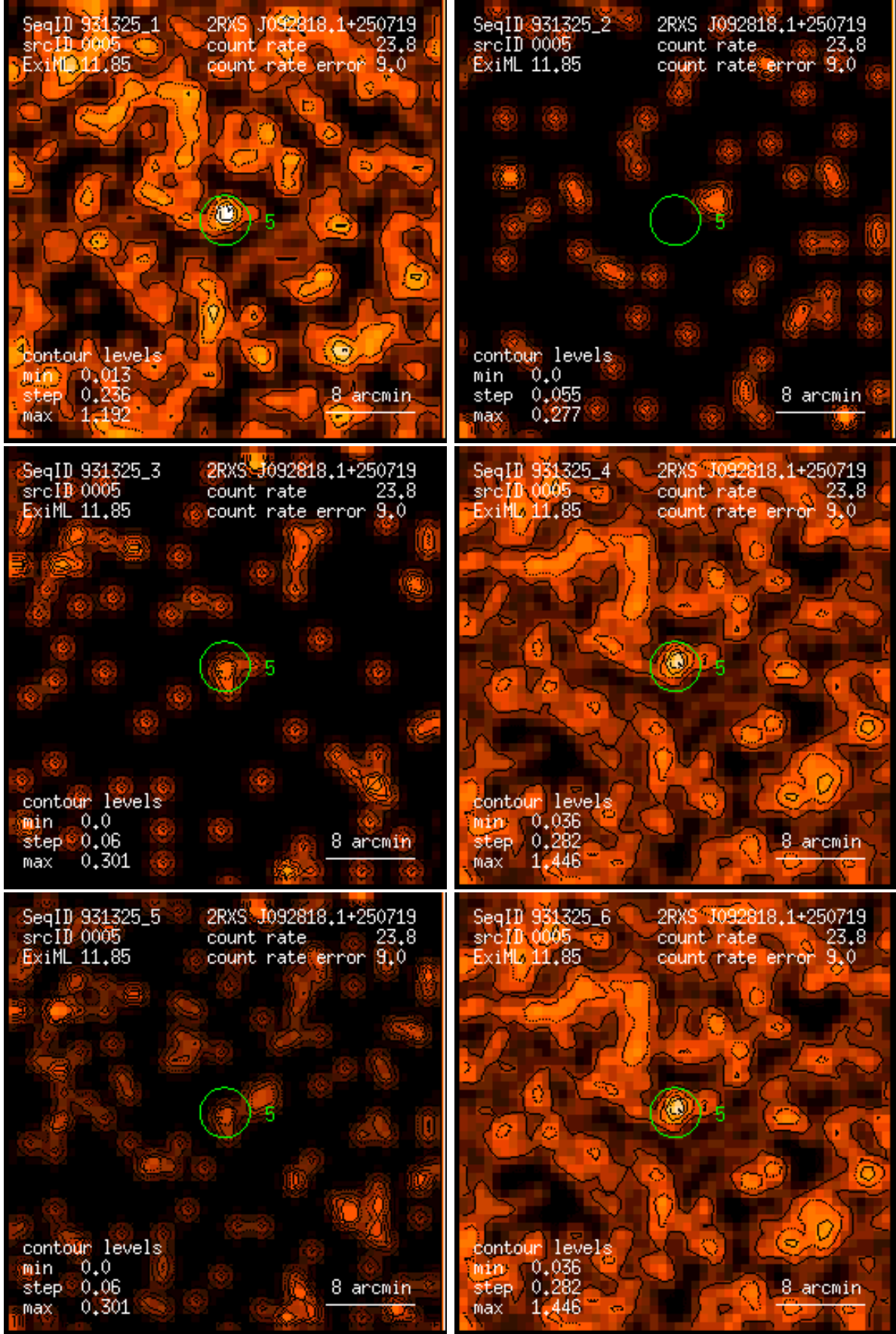
Figure 5: RASS 931325: detection 0005: band rate images, Gaussian filter: (1) PSPC channels 11 – 41, (2) 52 – 90, (3) 91 – 201, (4) 11 – 235, (5) 52 – 201, (6) 11 – 201. Broad band rates in counts/ks. Band rate contour levels in counts/ks/arcmin 2 .
