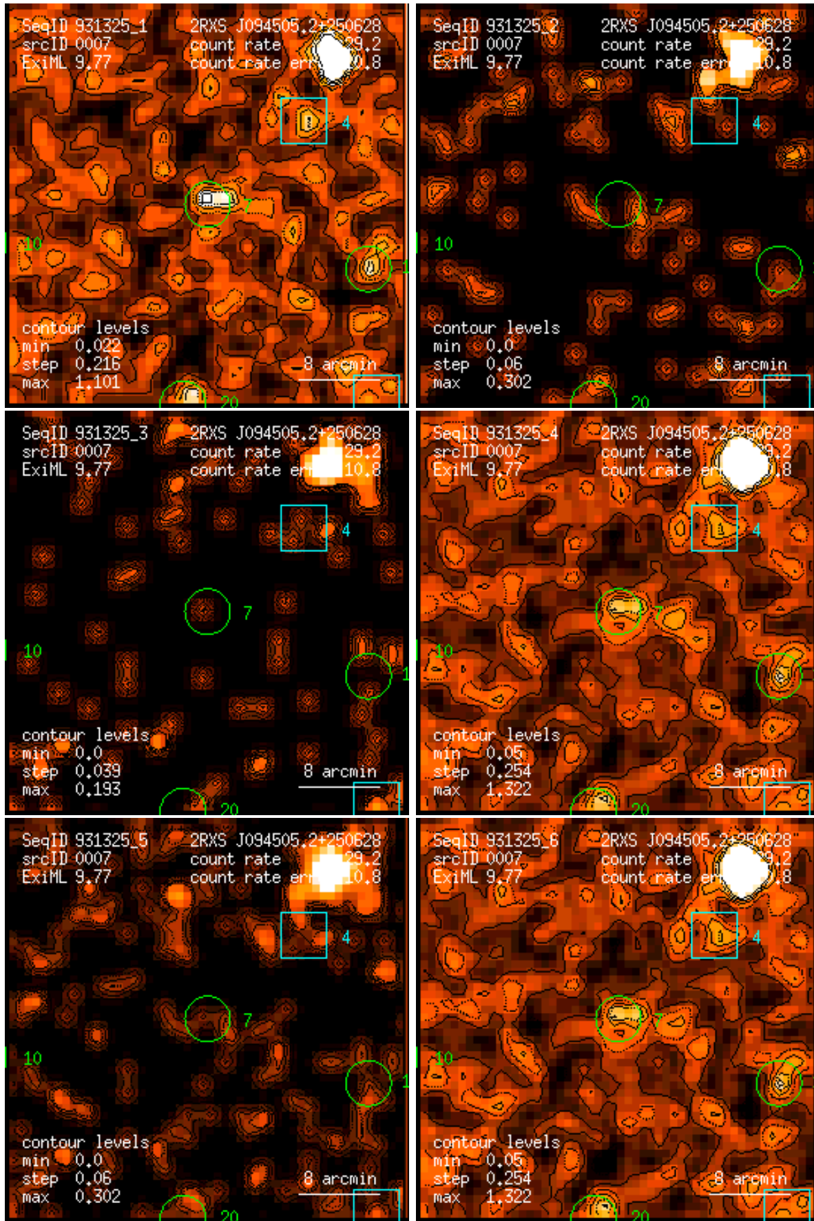
Figure 7: RASS 931325: detection 0007: band rate images, Gaussian filter: (1) PSPC channels 11 – 41, (2) 52 – 90, (3) 91 – 201, (4) 11 – 235, (5) 52 – 201, (6) 11 – 201. Broad band rates in counts/ks. Band rate contour levels in counts/ks/arcmin 2 .
