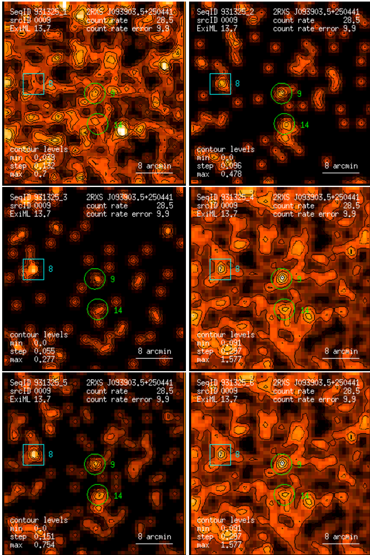
Figure 9: RASS 931325: detection 0009: band rate images, Gaussian filter: (1) PSPC channels 11 – 41, (2) 52 – 90, (3) 91 – 201, (4) 11 – 235, (5) 52 – 201, (6) 11 – 201. Broad band rates in counts/ks. Band rate contour levels in counts/ks/arcmin 2 .
