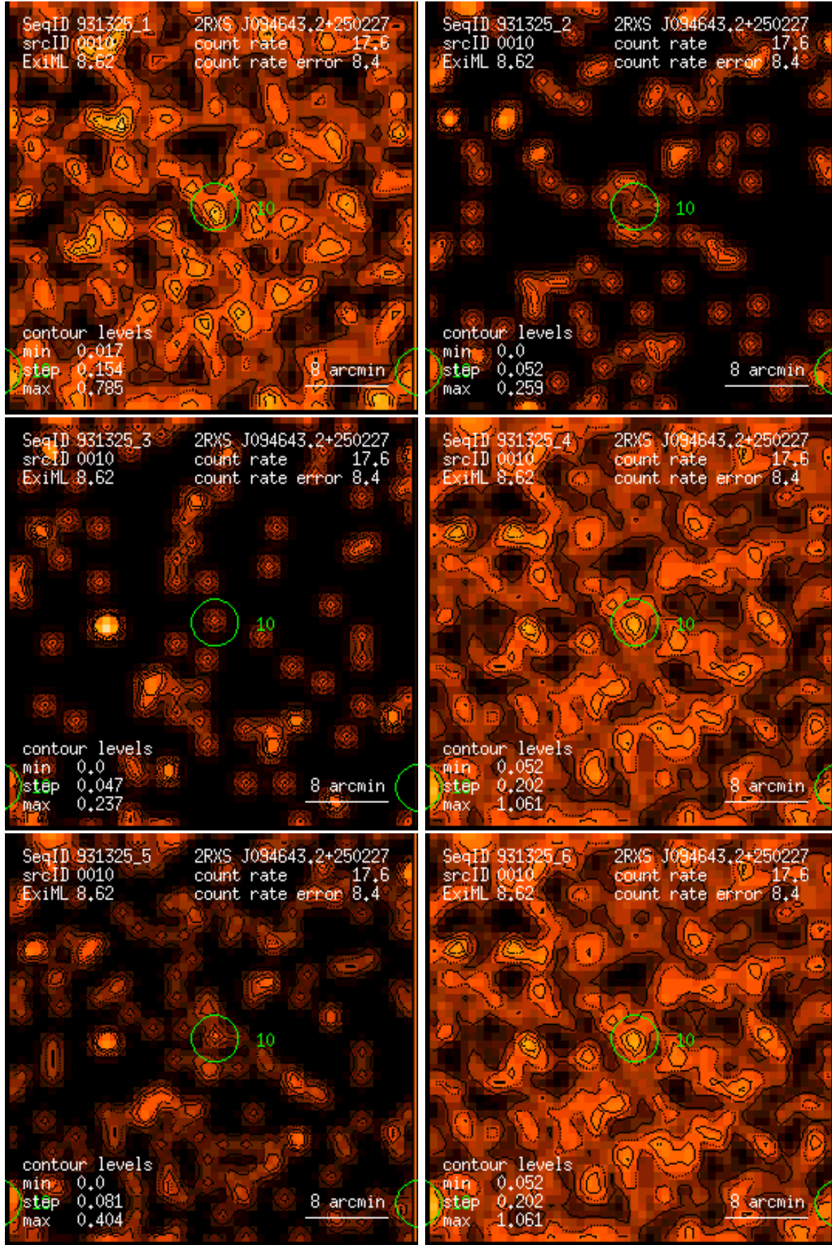
Figure 10: RASS 931325: detection 0010: band rate images, Gaussian filter: (1) PSPC channels 11 – 41, (2) 52 – 90, (3) 91 – 201, (4) 11 – 235, (5) 52 – 201, (6) 11 – 201. Broad band rates in counts/ks. Band rate contour levels in counts/ks/arcmin 2 .
