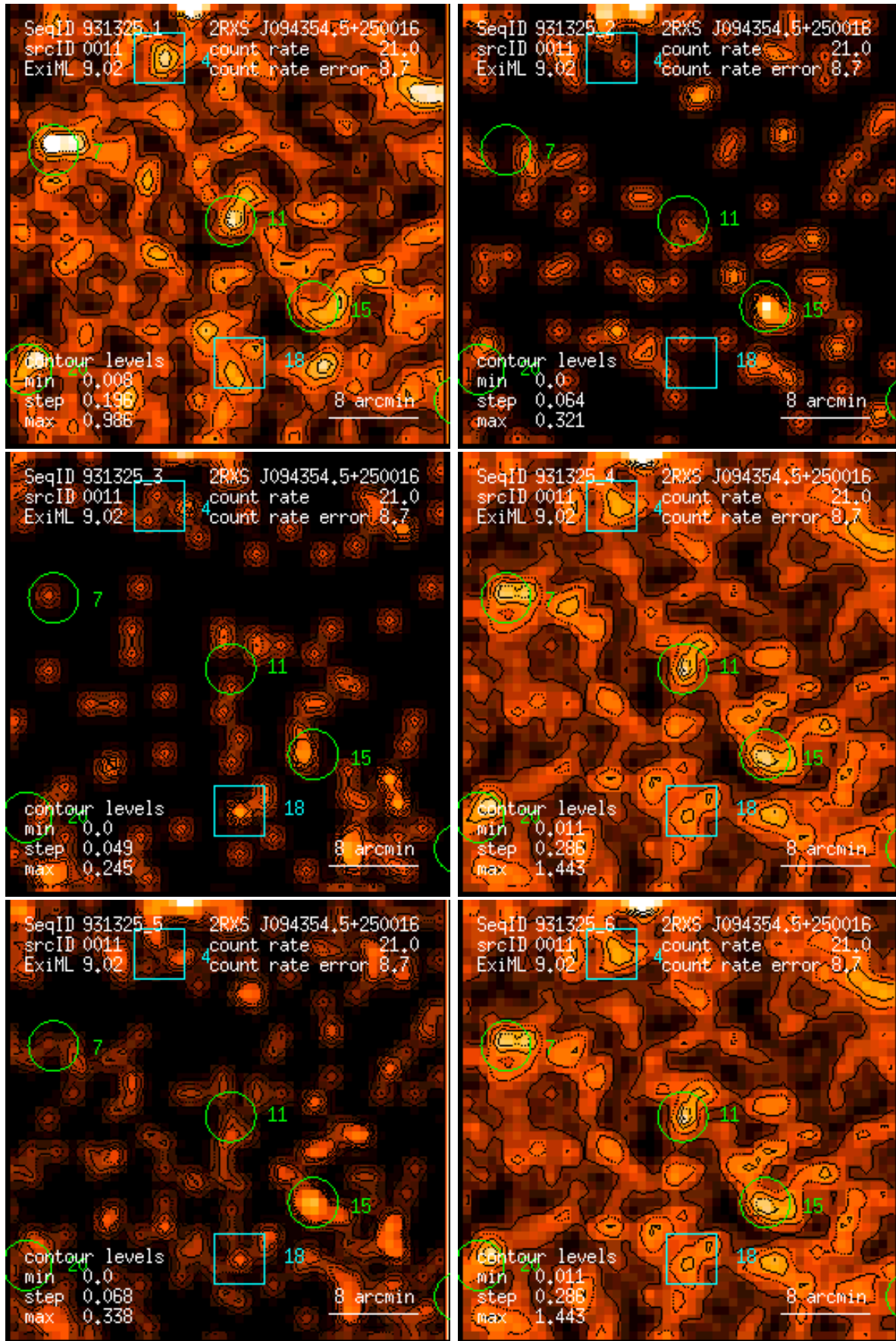
Figure 11: RASS 931325: detection 0011: band rate images, Gaussian filter: (1) PSPC channels 11 – 41, (2) 52 – 90, (3) 91 – 201, (4) 11 – 235, (5) 52 – 201, (6) 11 – 201. Broad band rates in counts/ks. Band rate contour levels in counts/ks/arcmin 2 .
