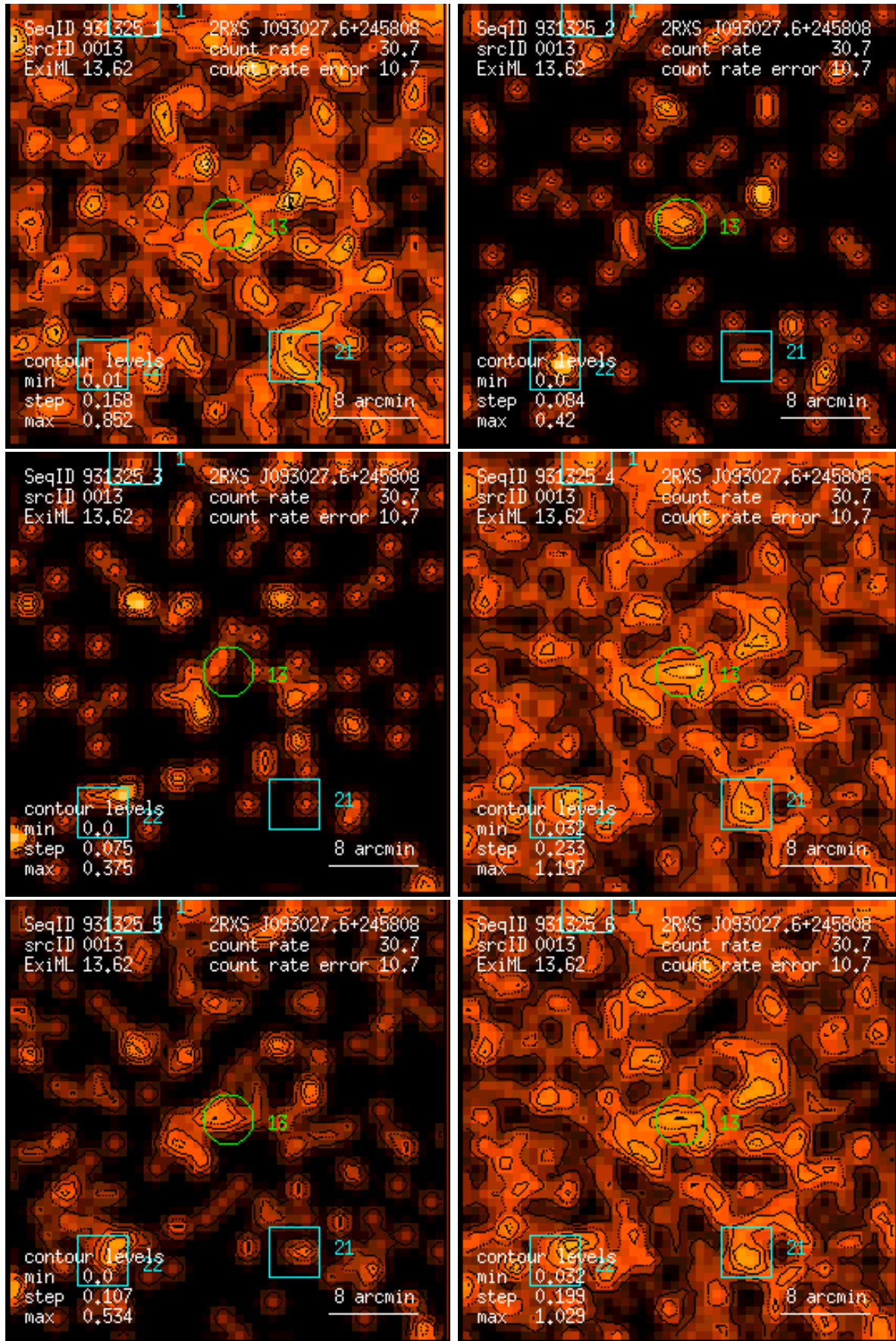
Figure 13: RASS 931325: detection 0013: band rate images, Gaussian filter: (1) PSPC channels 11 – 41, (2) 52 – 90, (3) 91 – 201, (4) 11 – 235, (5) 52 – 201, (6) 11 – 201. Broad band rates in counts/ks. Band rate contour levels in counts/ks/arcmin 2 .
