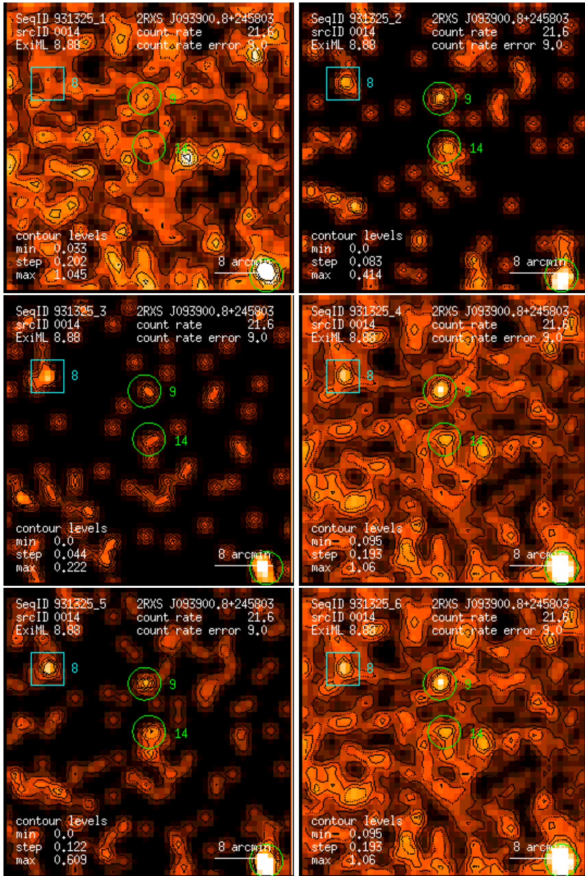
Figure 14: RASS 931325: detection 0014: band rate images, Gaussian filter: (1) PSPC channels 11 – 41, (2) 52 – 90, (3) 91 – 201, (4) 11 – 235, (5) 52 – 201, (6) 11 – 201. Broad band rates in counts/ks. Band rate contour levels in counts/ks/arcmin 2 .
