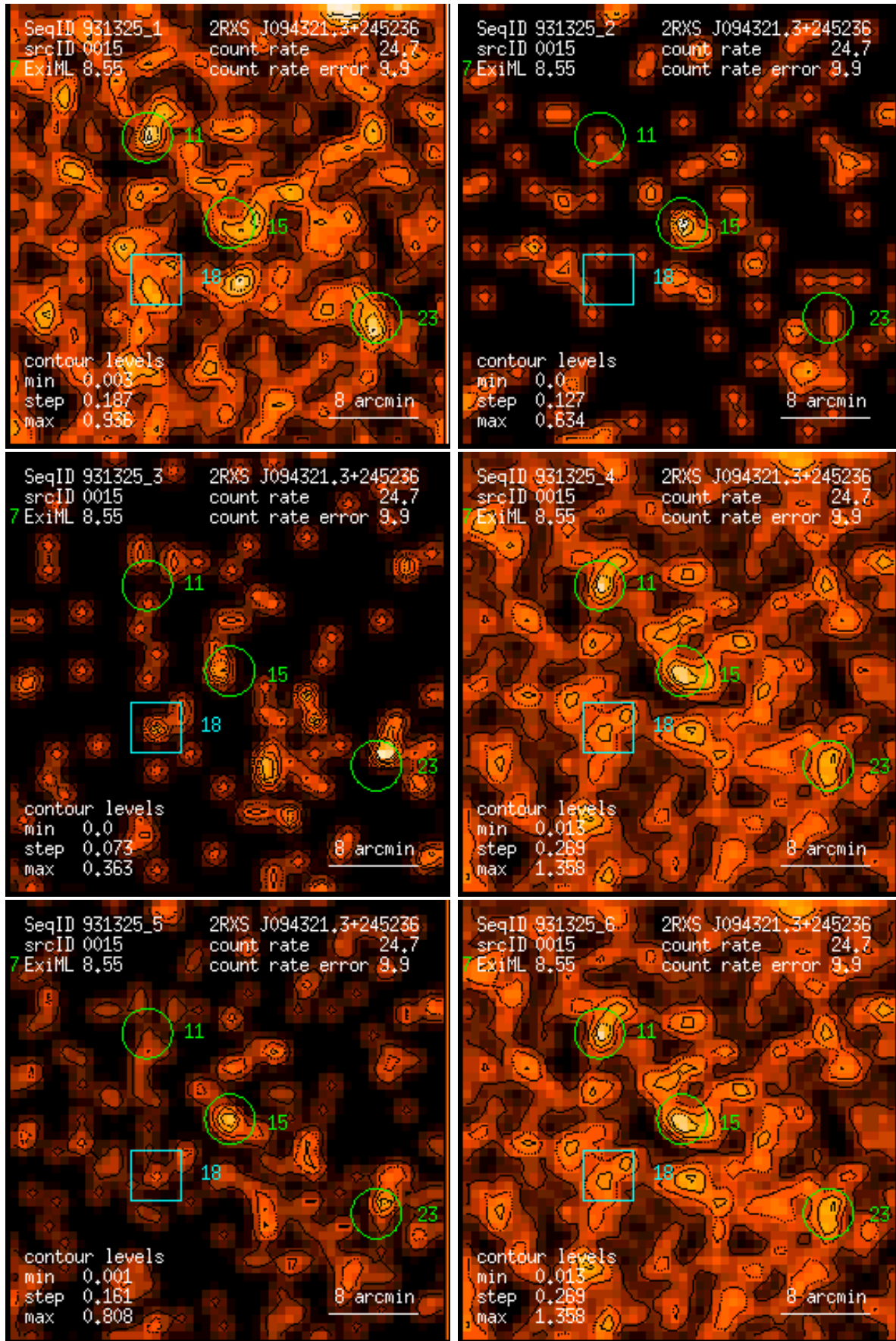
Figure 15: RASS 931325: detection 0015: band rate images, Gaussian filter: (1) PSPC channels 11 – 41, (2) 52 – 90, (3) 91 – 201, (4) 11 – 235, (5) 52 – 201, (6) 11 – 201. Broad band rates in counts/ks. Band rate contour levels in counts/ks/arcmin 2 .
