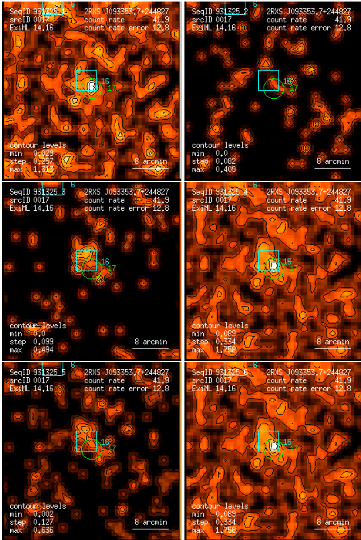
Figure 17: RASS 931325: detection 0017: band rate images, Gaussian filter: (1) PSPC channels 11 – 41, (2) 52 – 90, (3) 91 – 201, (4) 11 – 235, (5) 52 – 201, (6) 11 – 201. Broad band rates in counts/ks. Band rate contour levels in counts/ks/arcmin 2 .
