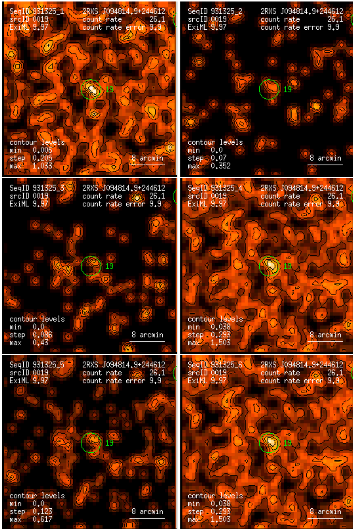
Figure 19: RASS 931325: detection 0019: band rate images, Gaussian filter: (1) PSPC channels 11 – 41, (2) 52 – 90, (3) 91 – 201, (4) 11 – 235, (5) 52 – 201, (6) 11 – 201. Broad band rates in counts/ks. Band rate contour levels in counts/ks/arcmin 2 .
