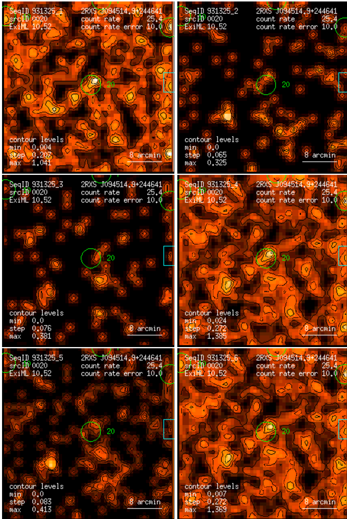
Figure 20: RASS 931325: detection 0020: band rate images, Gaussian filter: (1) PSPC channels 11 – 41, (2) 52 – 90, (3) 91 – 201, (4) 11 – 235, (5) 52 – 201, (6) 11 – 201. Broad band rates in counts/ks. Band rate contour levels in counts/ks/arcmin 2 .
