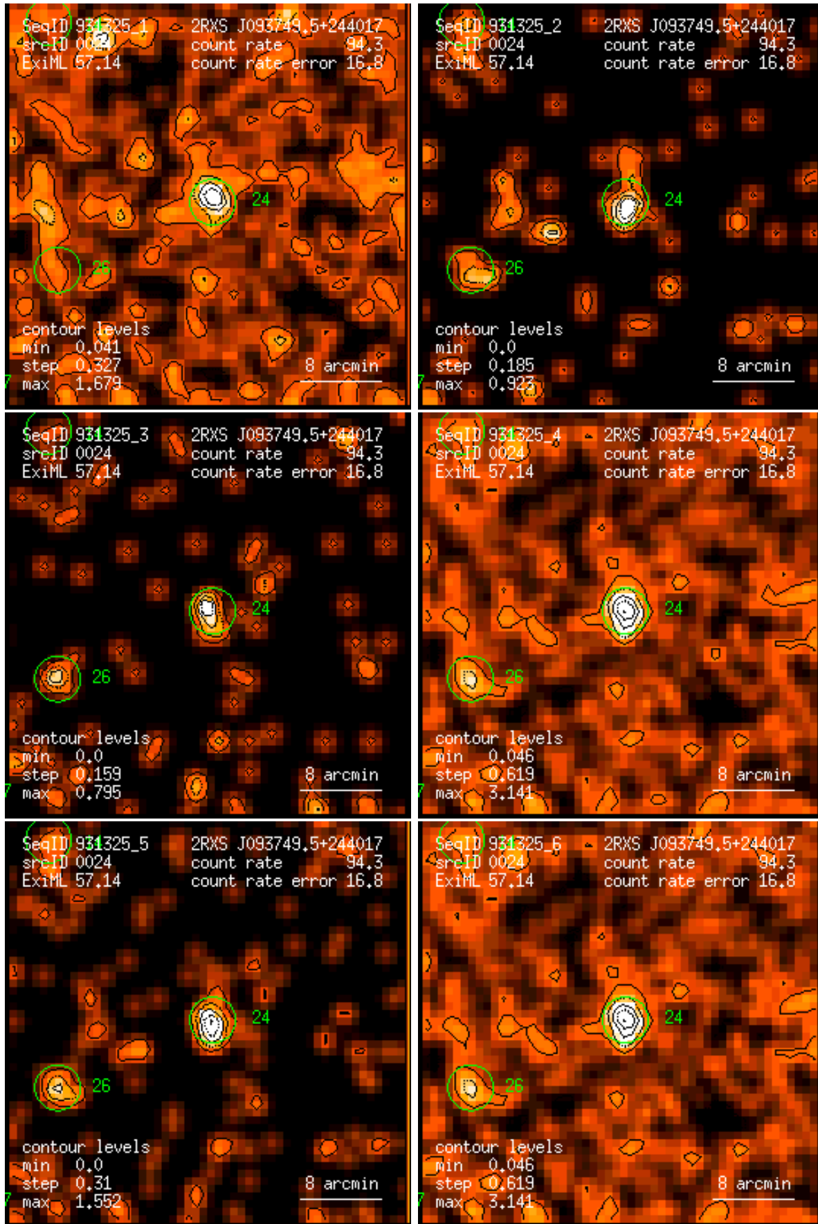
Figure 24: RASS 931325: detection 0024: band rate images, Gaussian filter: (1) PSPC channels 11 – 41, (2) 52 – 90, (3) 91 – 201, (4) 11 – 235, (5) 52 – 201, (6) 11 – 201. Broad band rates in counts/ks. Band rate contour levels in counts/ks/arcmin 2 .
