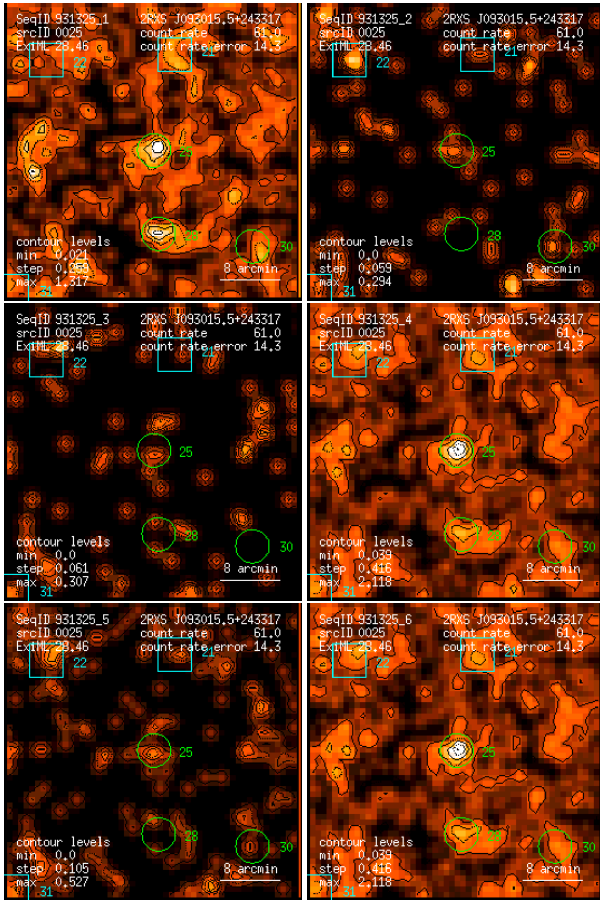
Figure 25: RASS 931325: detection 0025: band rate images, Gaussian filter: (1) PSPC channels 11 – 41, (2) 52 – 90, (3) 91 – 201, (4) 11 – 235, (5) 52 – 201, (6) 11 – 201. Broad band rates in counts/ks. Band rate contour levels in counts/ks/arcmin 2 .
