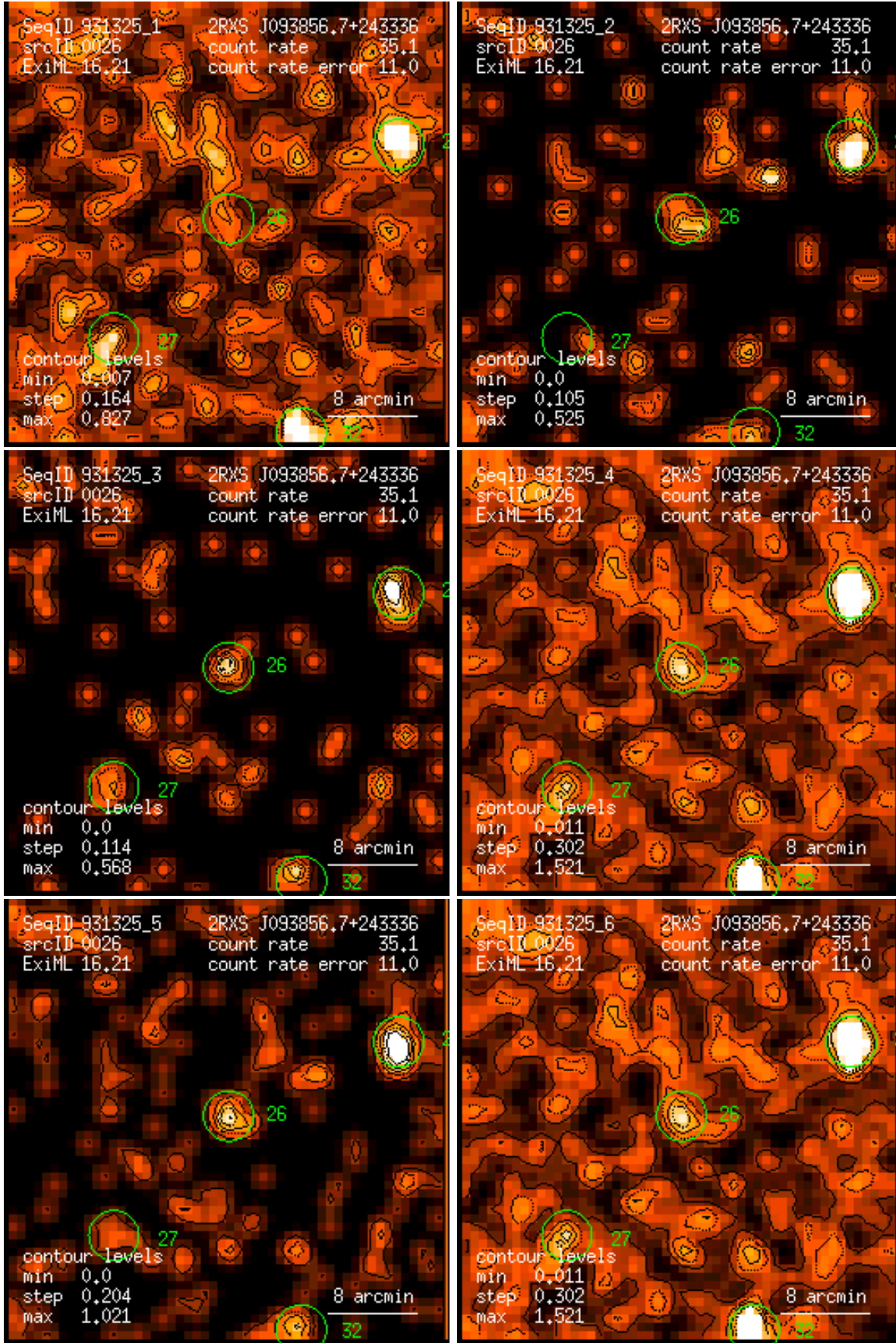
Figure 26: RASS 931325: detection 0026: band rate images, Gaussian filter: (1) PSPC channels 11 – 41, (2) 52 – 90, (3) 91 – 201, (4) 11 – 235, (5) 52 – 201, (6) 11 – 201. Broad band rates in counts/ks. Band rate contour levels in counts/ks/arcmin 2 .
