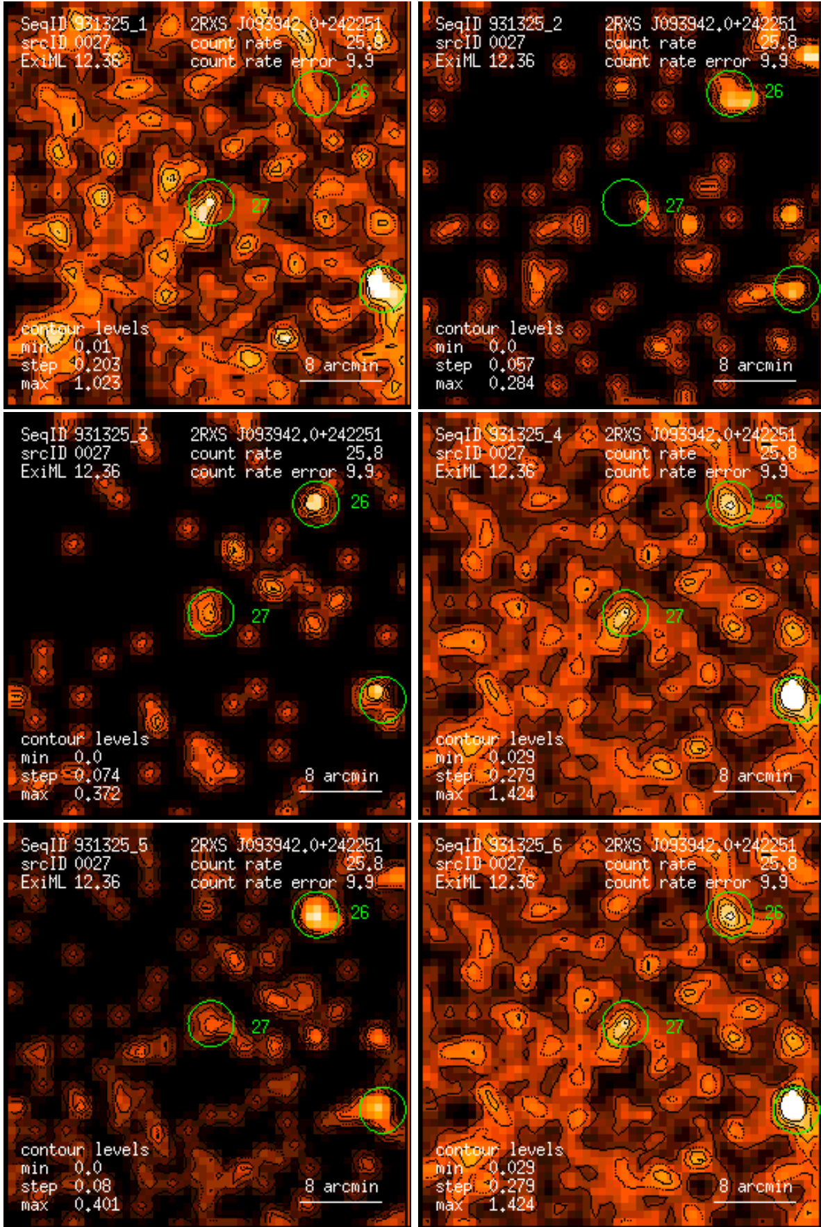
Figure 27: RASS 931325: detection 0027: band rate images, Gaussian filter: (1) PSPC channels 11 – 41, (2) 52 – 90, (3) 91 – 201, (4) 11 – 235, (5) 52 – 201, (6) 11 – 201. Broad band rates in counts/ks. Band rate contour levels in counts/ks/arcmin 2 .
