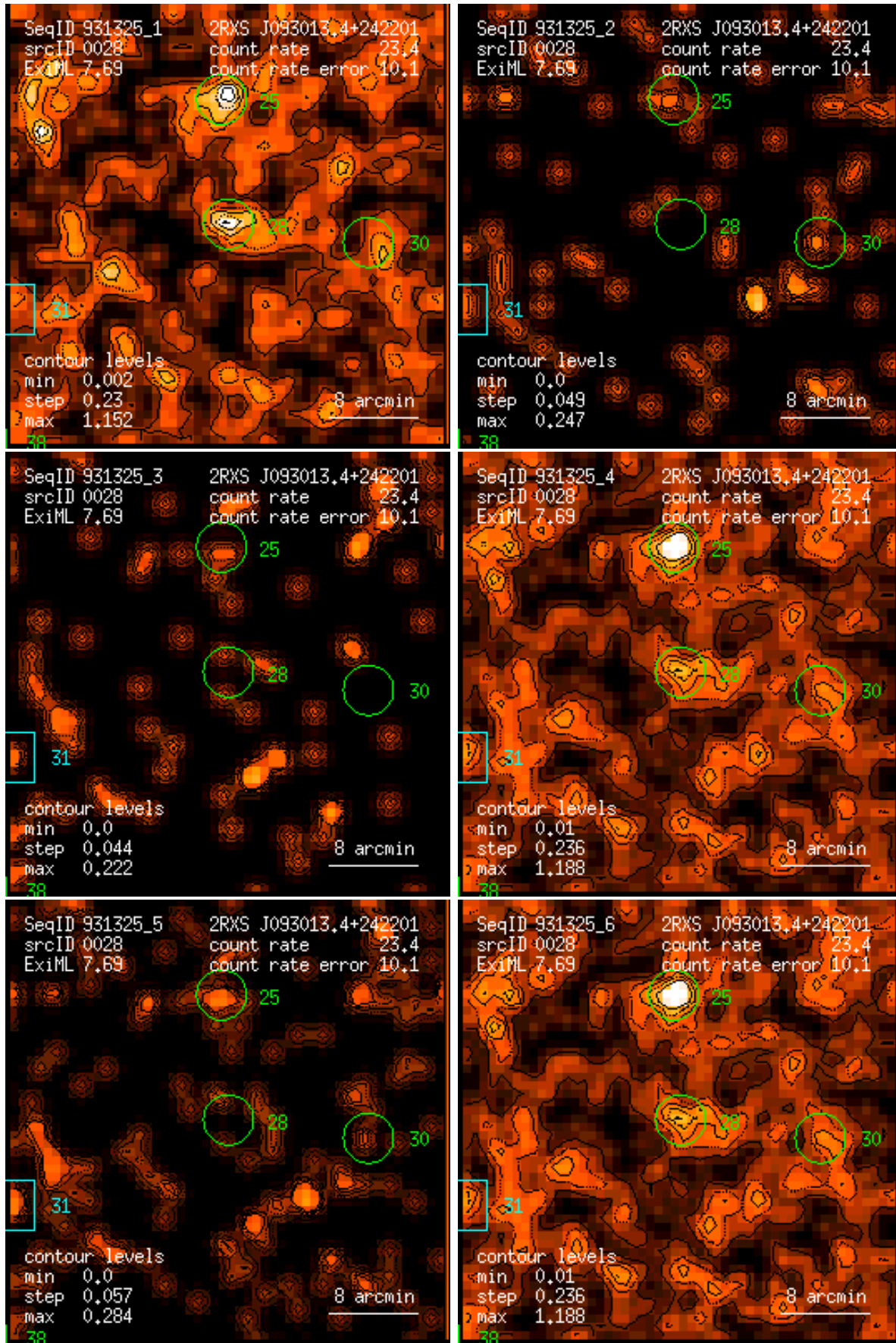
Figure 28: RASS 931325: detection 0028: band rate images, Gaussian filter: (1) PSPC channels 11 – 41, (2) 52 – 90, (3) 91 – 201, (4) 11 – 235, (5) 52 – 201, (6) 11 – 201. Broad band rates in counts/ks. Band rate contour levels in counts/ks/arcmin 2 .
