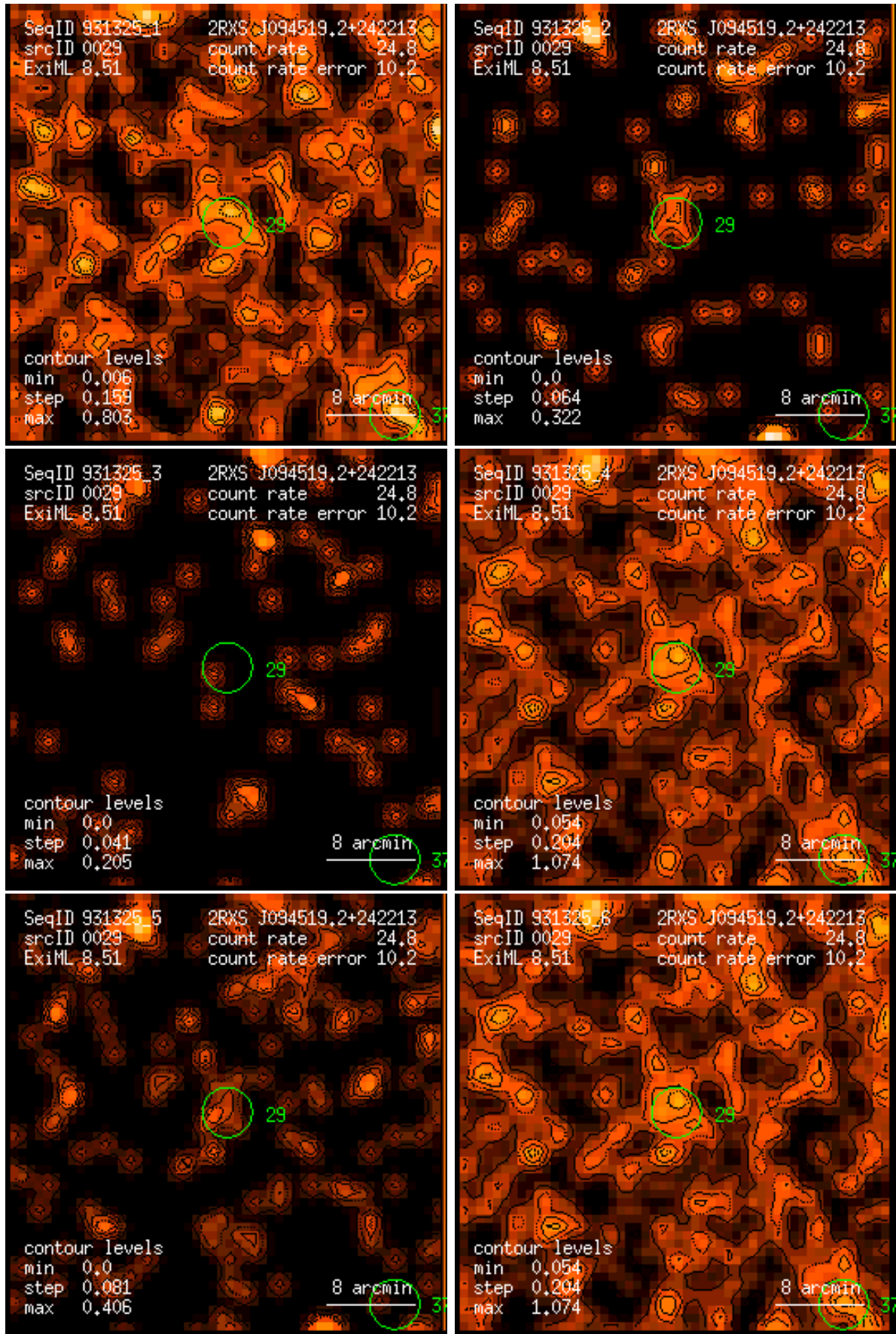
Figure 29: RASS 931325: detection 0029: band rate images, Gaussian filter: (1) PSPC channels 11 – 41, (2) 52 – 90, (3) 91 – 201, (4) 11 – 235, (5) 52 – 201, (6) 11 – 201. Broad band rates in counts/ks. Band rate contour levels in counts/ks/arcmin 2 .
