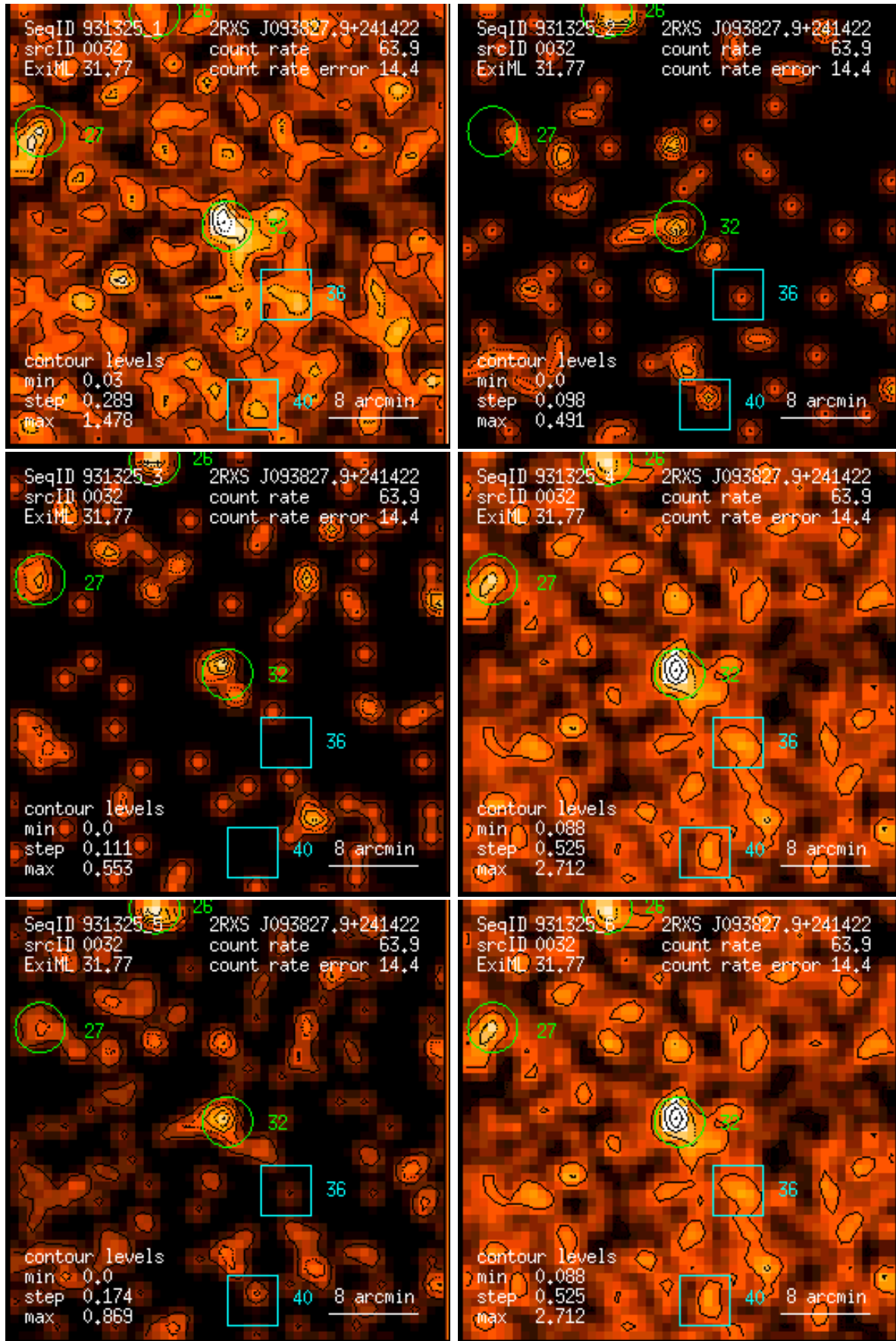
Figure 32: RASS 931325: detection 0032: band rate images, Gaussian filter: (1) PSPC channels 11 – 41, (2) 52 – 90, (3) 91 – 201, (4) 11 – 235, (5) 52 – 201, (6) 11 – 201. Broad band rates in counts/ks. Band rate contour levels in counts/ks/arcmin 2 .
