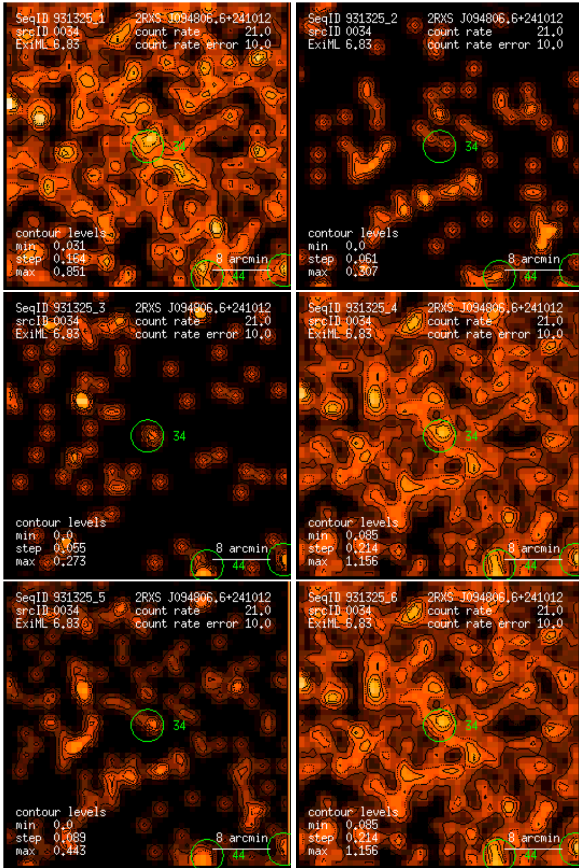
Figure 34: RASS 931325: detection 0034: band rate images, Gaussian filter: (1) PSPC channels 11 – 41, (2) 52 – 90, (3) 91 – 201, (4) 11 – 235, (5) 52 – 201, (6) 11 – 201. Broad band rates in counts/ks. Band rate contour levels in counts/ks/arcmin 2 .
