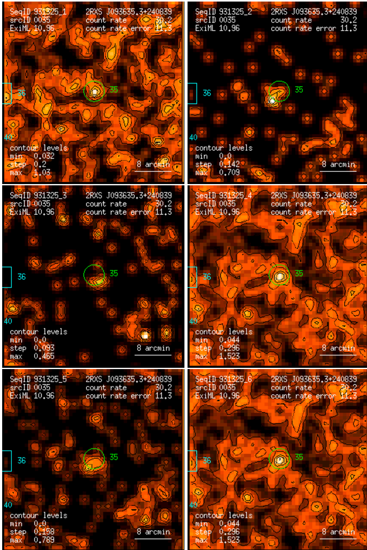
Figure 35: RASS 931325: detection 0035: band rate images, Gaussian filter: (1) PSPC channels 11 – 41, (2) 52 – 90, (3) 91 – 201, (4) 11 – 235, (5) 52 – 201, (6) 11 – 201. Broad band rates in counts/ks. Band rate contour levels in counts/ks/arcmin 2 .
