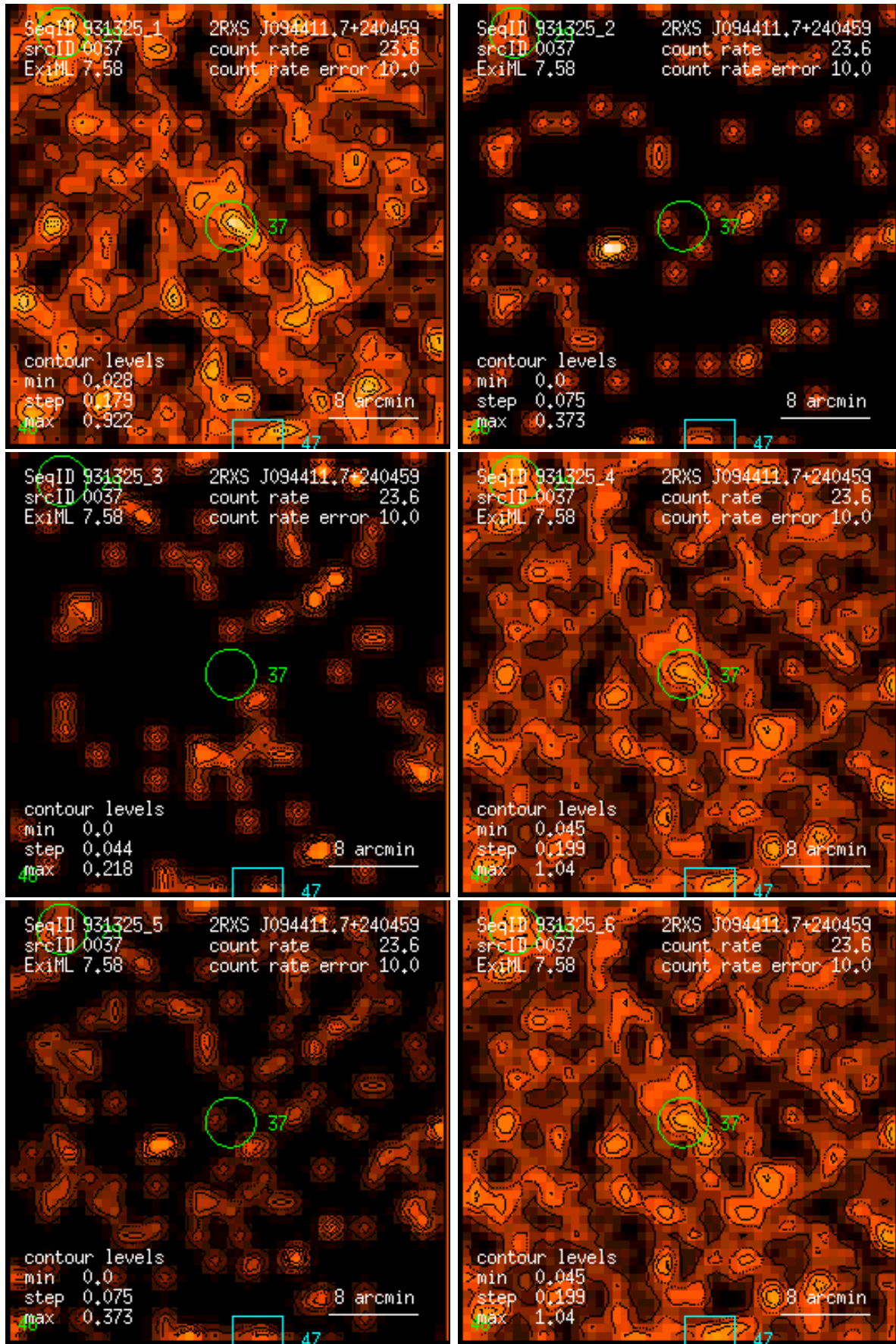
Figure 37: RASS 931325: detection 0037: band rate images, Gaussian filter: (1) PSPC channels 11 – 41, (2) 52 – 90, (3) 91 – 201, (4) 11 – 235, (5) 52 – 201, (6) 11 – 201. Broad band rates in counts/ks. Band rate contour levels in counts/ks/arcmin 2 .
